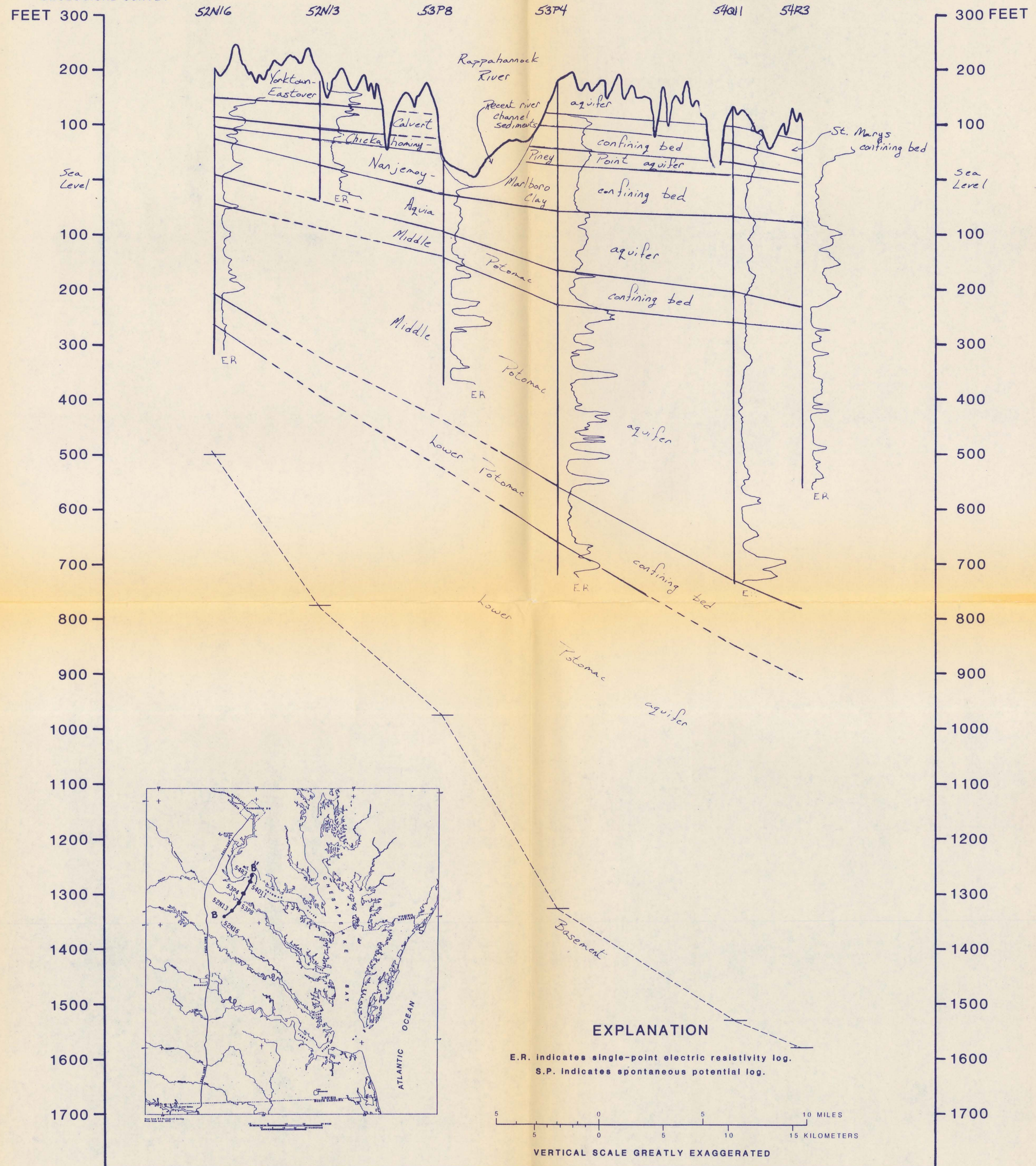
HYDROGEOLOGIC SECTION B-B' FROM WELL 52N16, CAROLINE COUNTY, TO WELL 54R3, KING GEORGE COUNTY, VIRGINIA.
