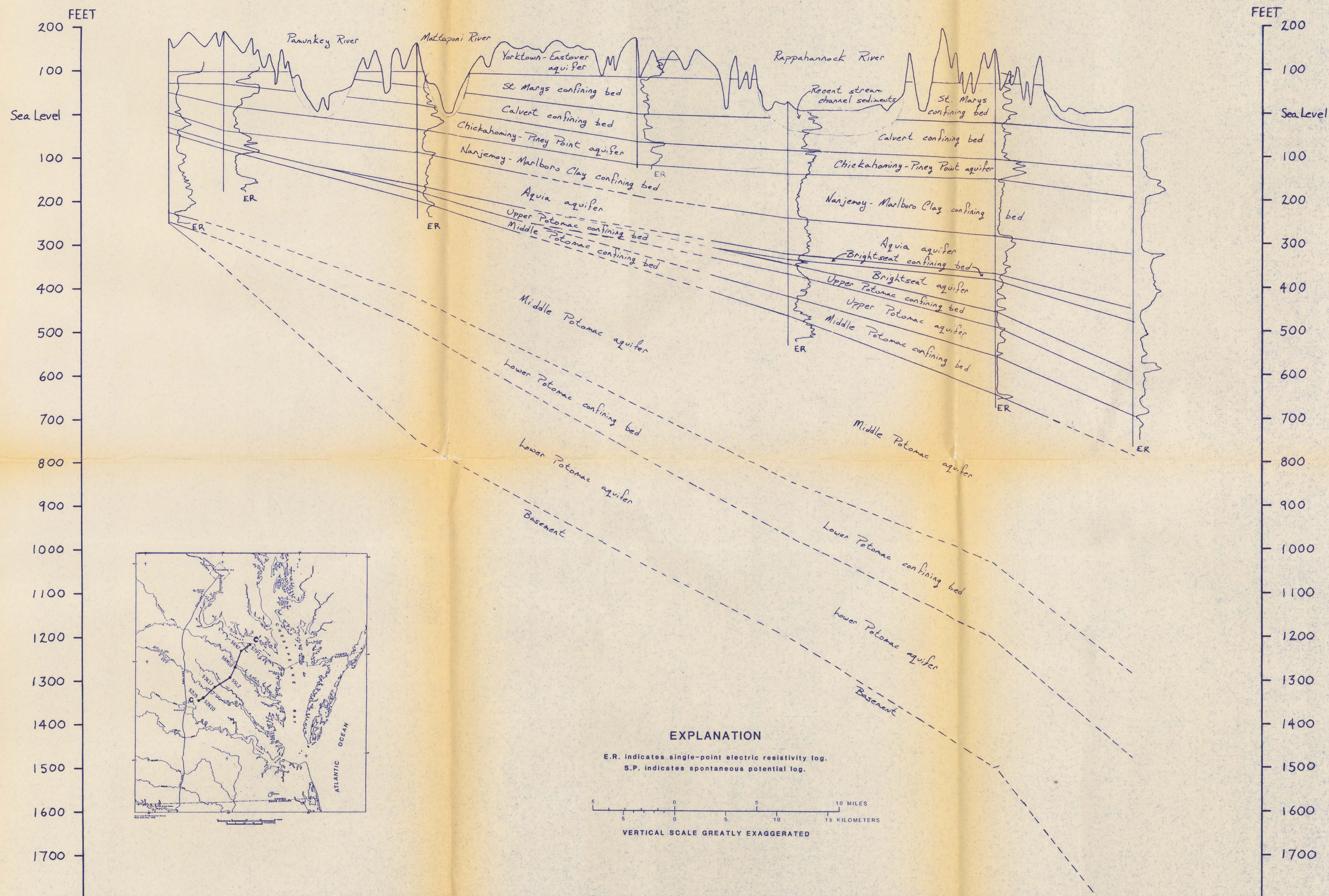
HYDROGEOLOGIC SECTION C-C' FROM WELL 52J5 HANOVER COUNTY, TO WELL 57PI, WESTMORELAND COUNTY, VIRGINIA.
