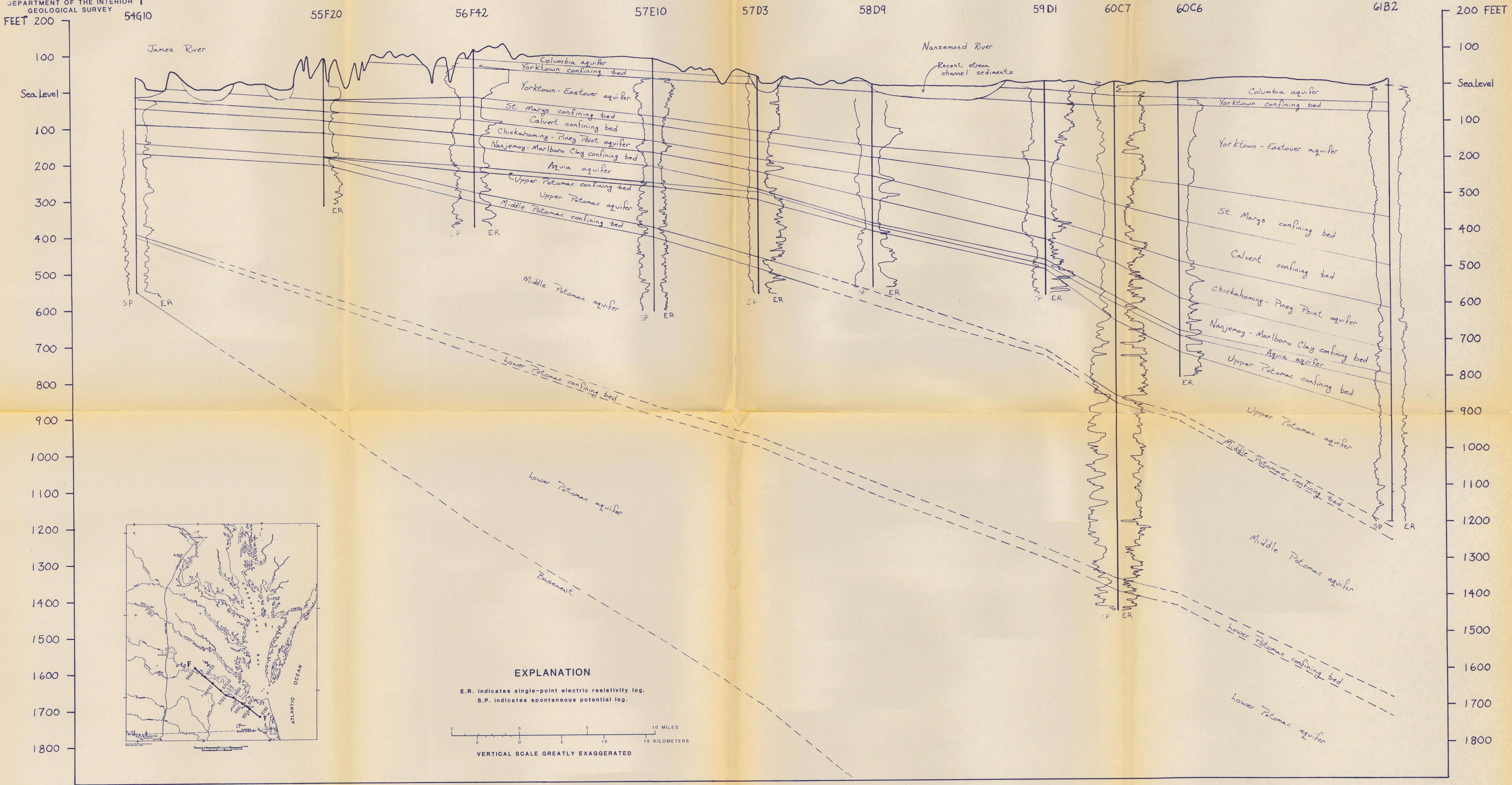
HYDROGEOLOGIC SECTION F-F' FROM WELL 54G10, CHARLES CITY COUNTY, TO WELL 61B2, CHESAPEAKE, VIRGINIA.
