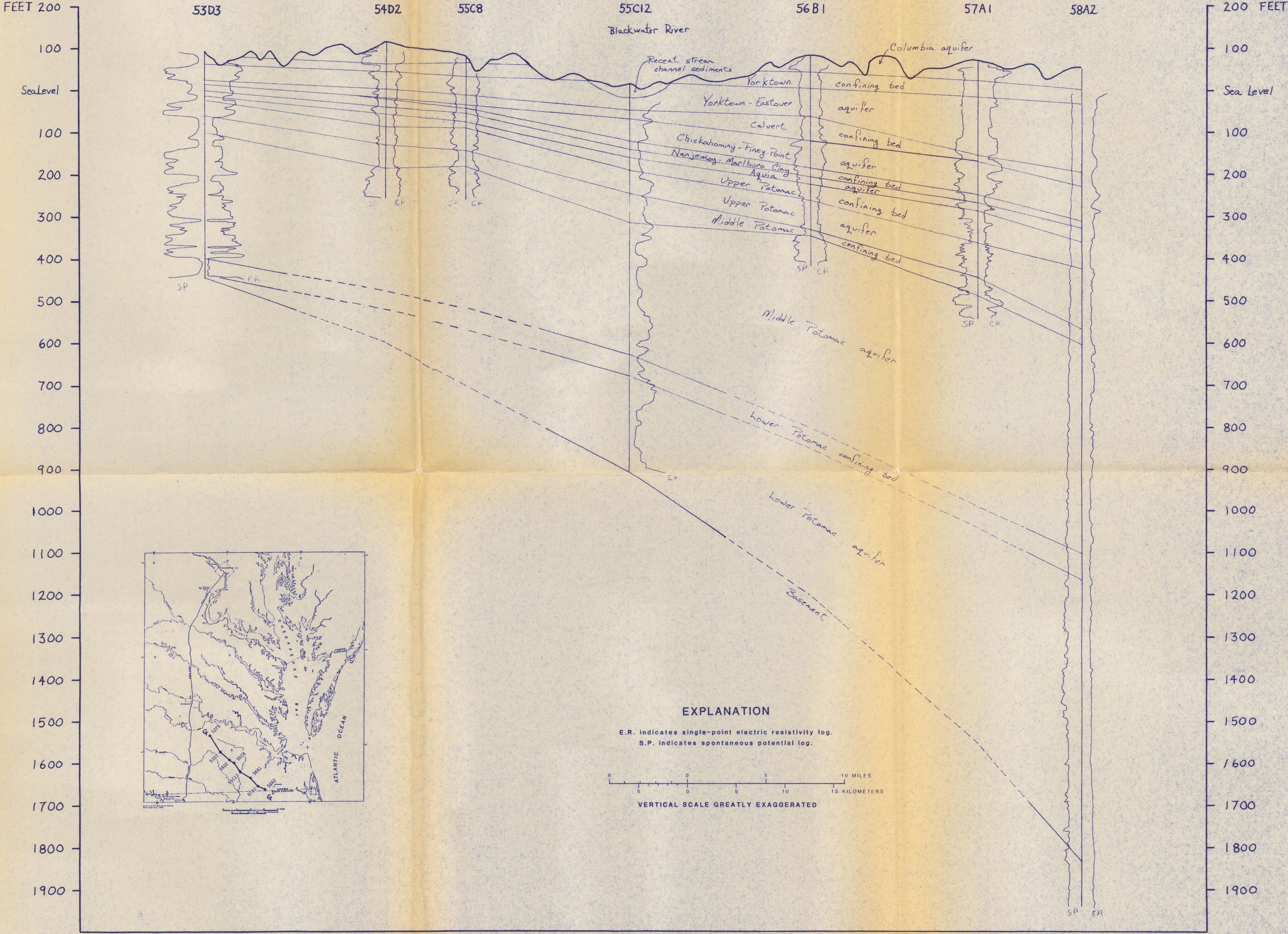
HYDROGEOLOGIC SECTION G-G' FROM WELL 53D3 SUSSEX COUNTY, TO WELL 58A2 SUFFOLK, VIRGINIA.
