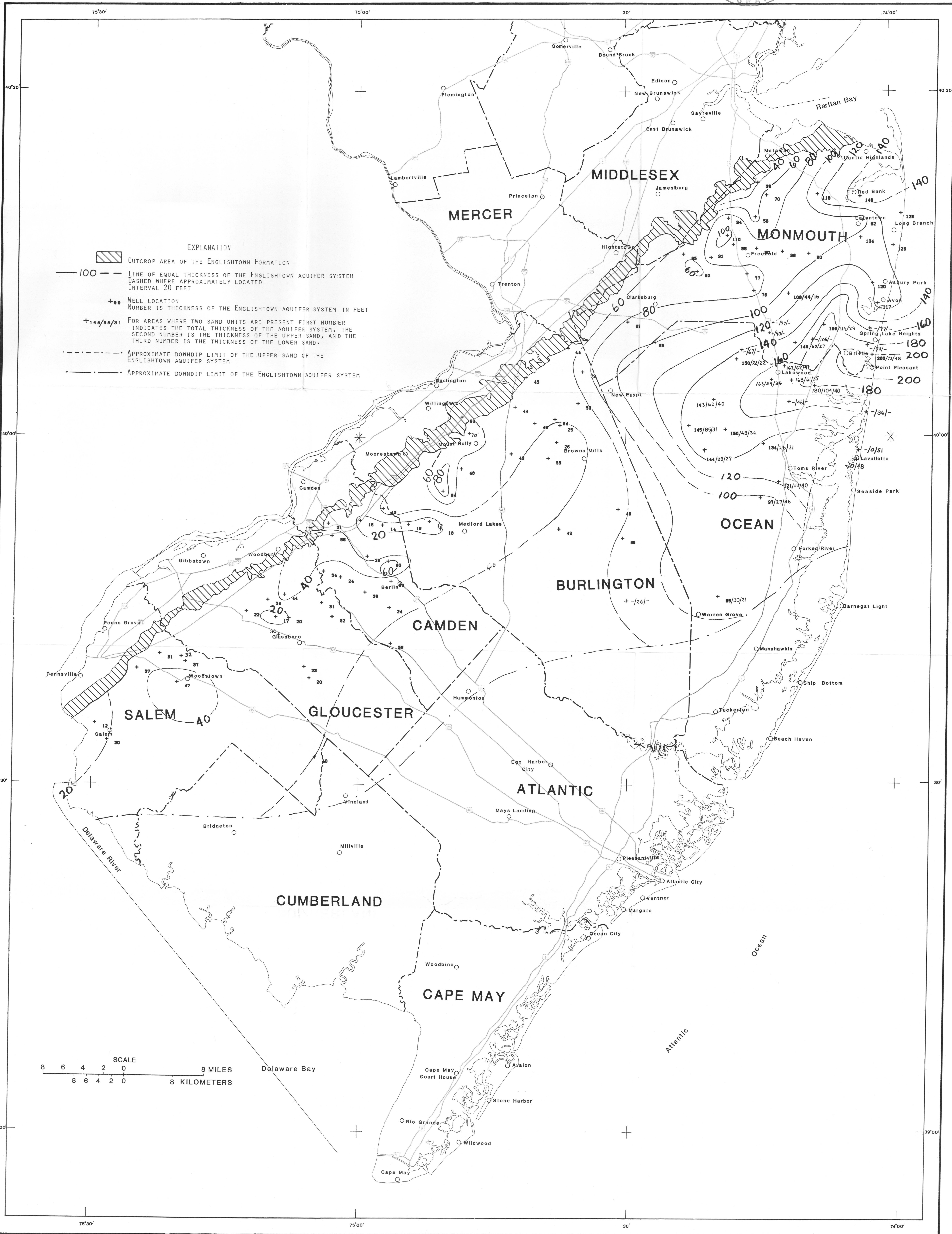
THICKNESS OF THE ENGLISHTOWN AQUIFER SYSTEM, NEW JERSEY.
