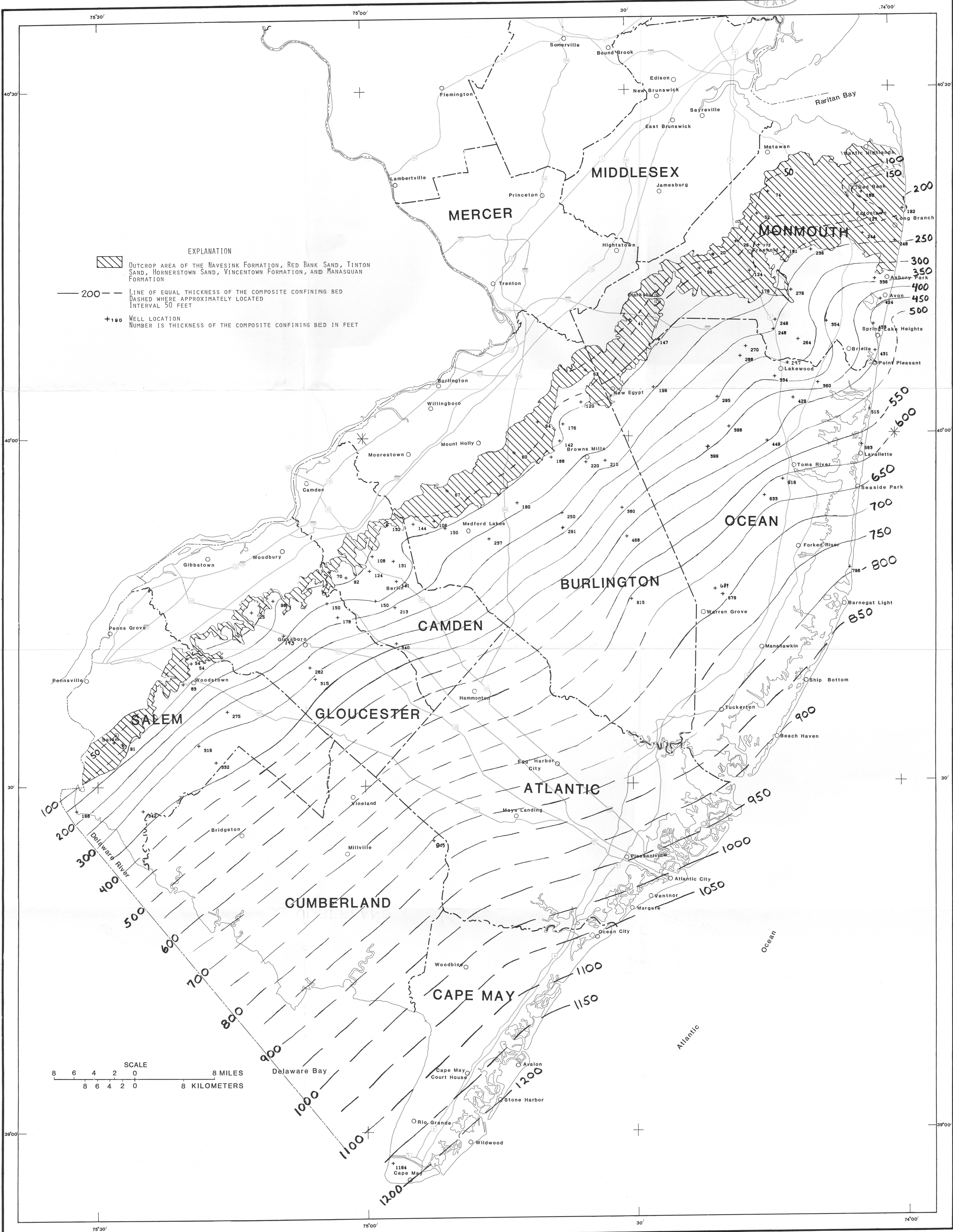
THICKNESS OF THE COMPOSITE CONFINING BED, NEW JERSEY.
