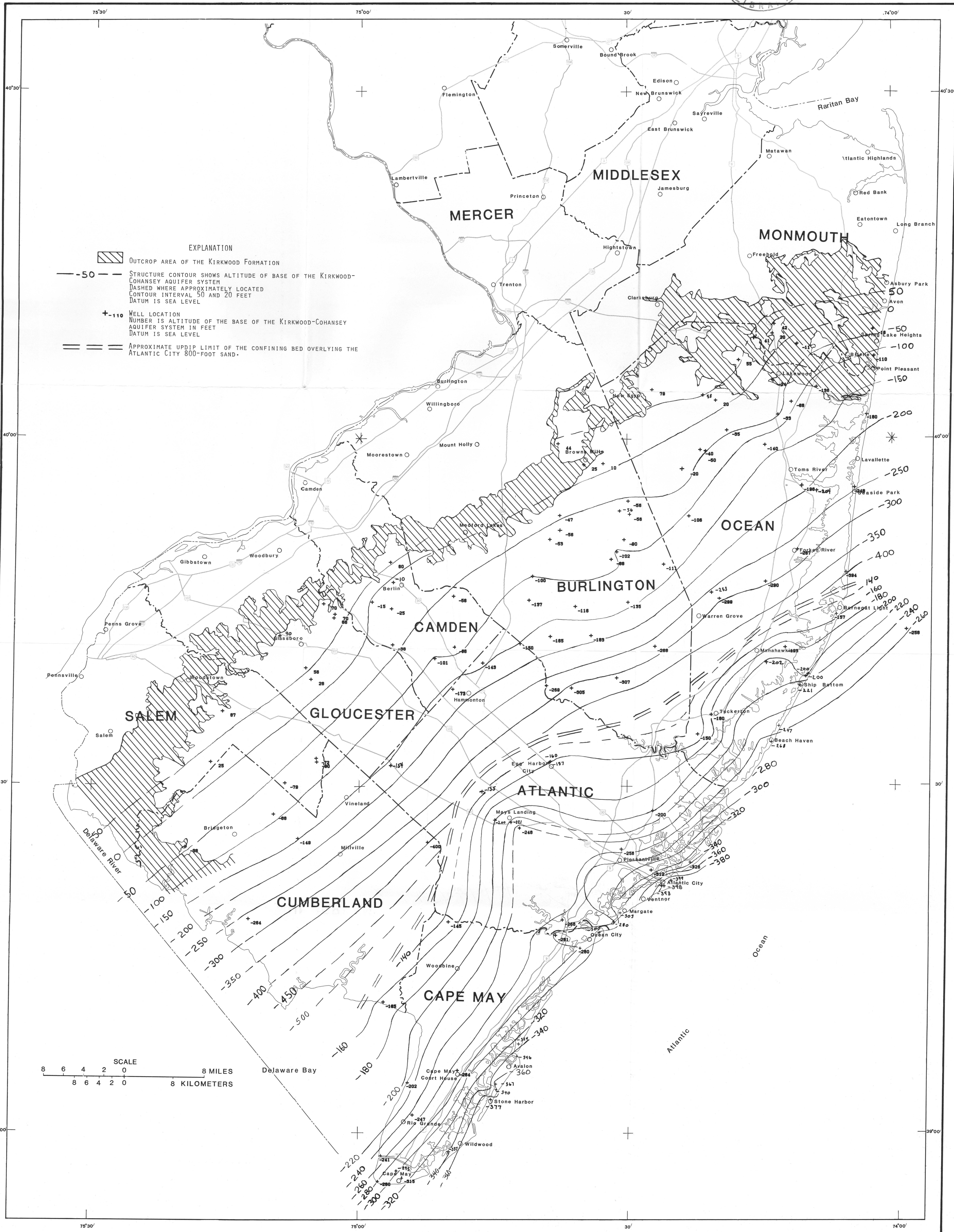
STRUCTURE CONTOURS OF THE BASE OF THE KIRKWOOD-COHANSEY AQUIFER SYSTEM, NEW JERSEY.
