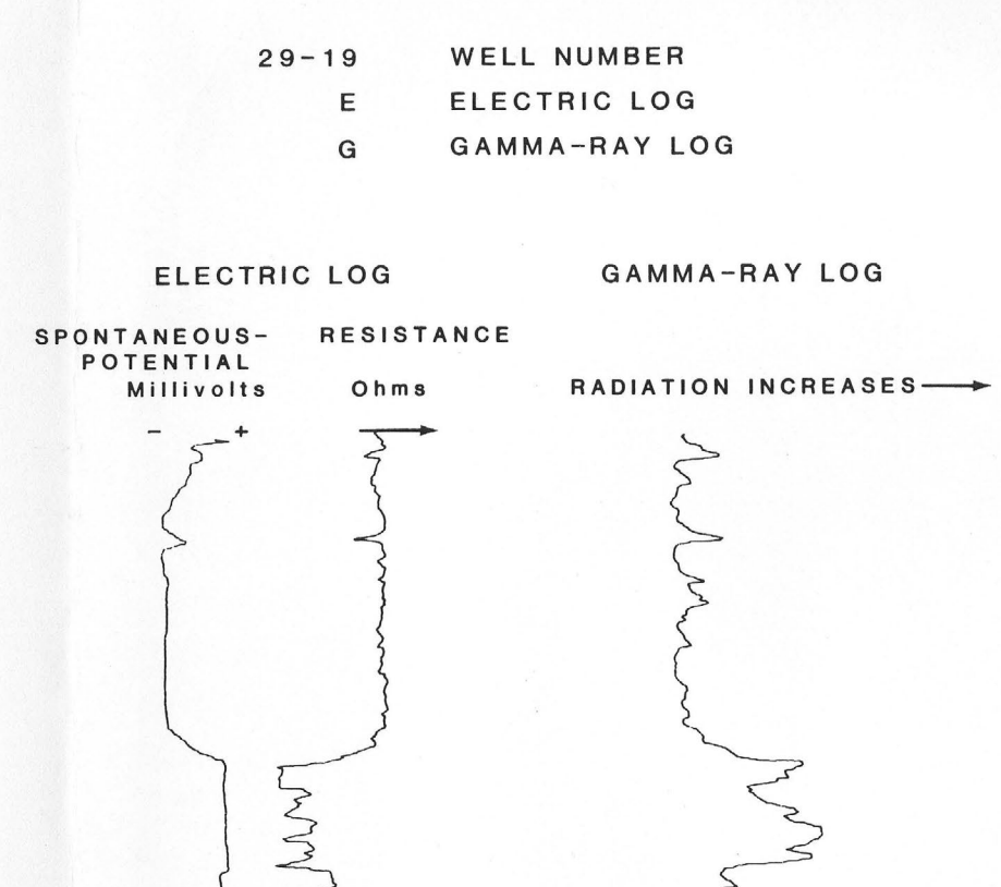
HYDROGEOLOGIC SECTIONS, COASTAL PLAIN, NEW JERSEY F-F' through J-J'
