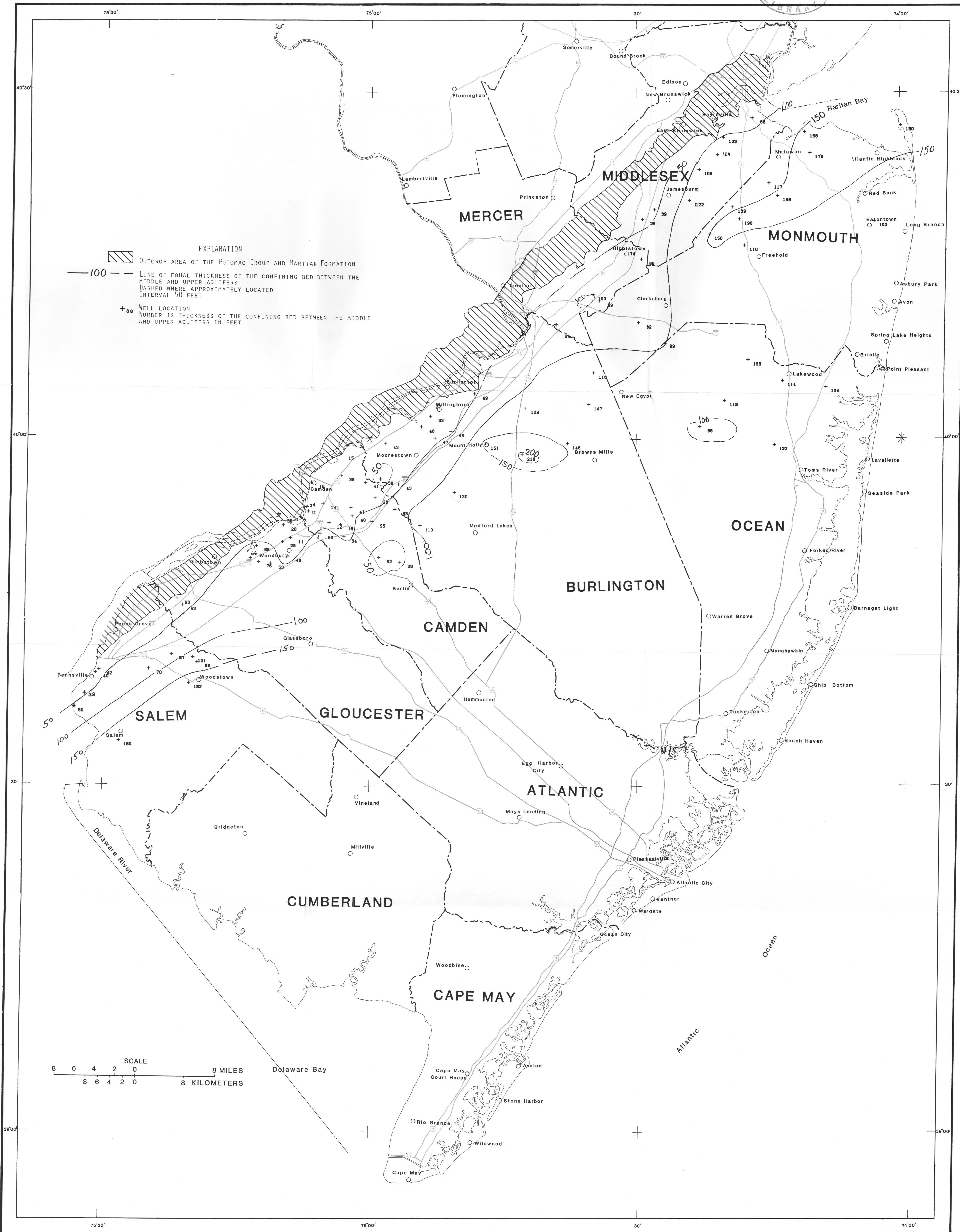
THICKNESS OF THE CONFINING BED BETWEEN THE MIDDLE AND UPPER AQUIFERS OF THE POTOMAC-RARITAN-MAGOTHY AQUIFER SYSTEM, NEW JERSEY.
