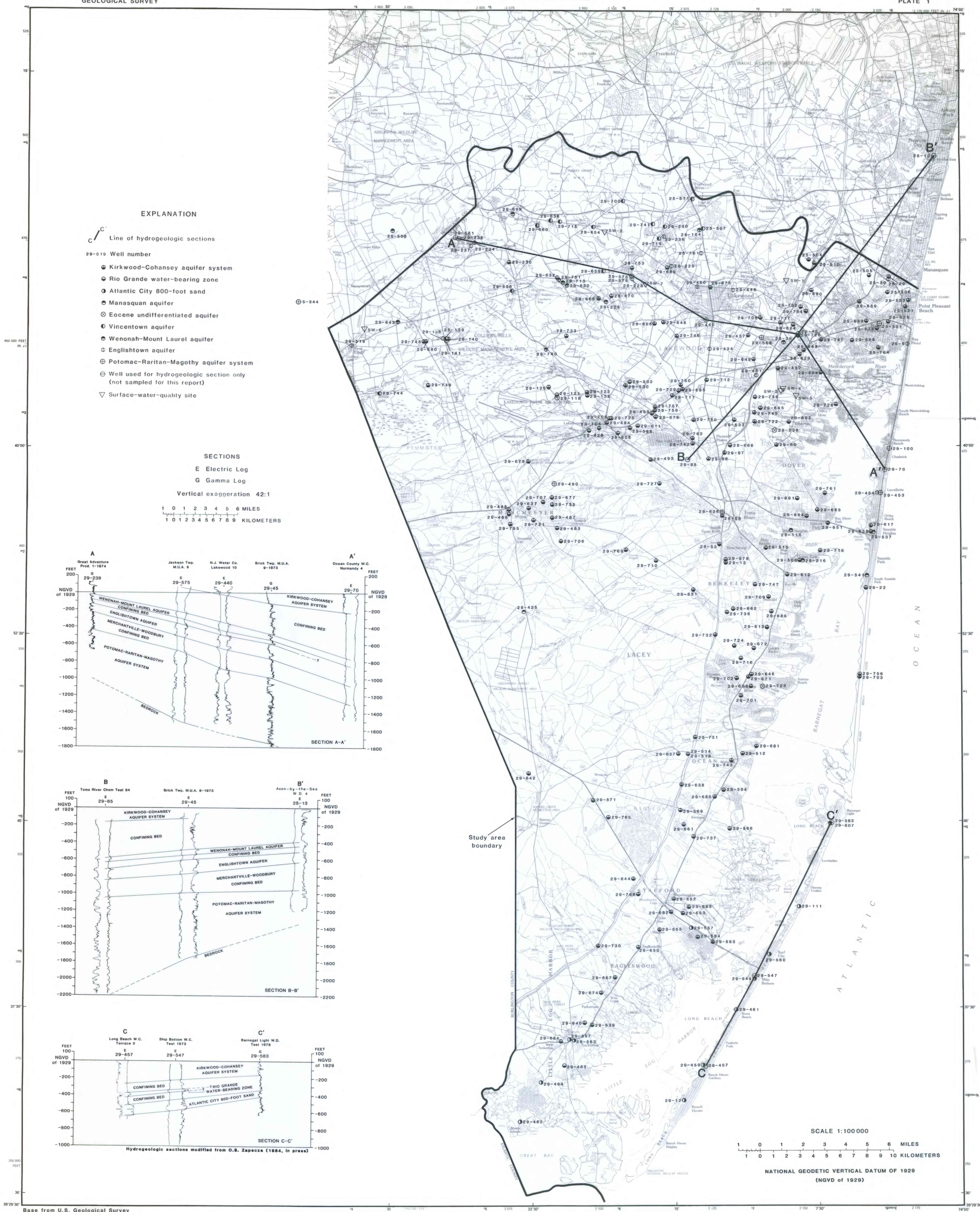
EAST-CENTRAL NEW JERSEY SHOWING SAMPLING SITES AND HYDROGEOLOGIC SECTIONS
