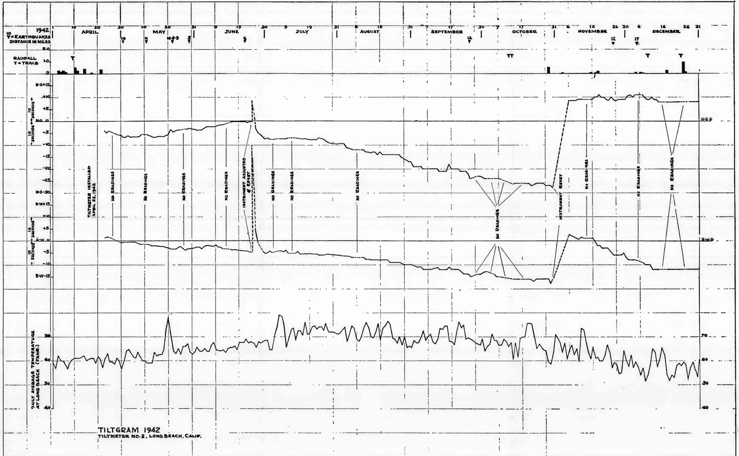
FIGURE 12.—Long Beach tilt-graph for 1942.
