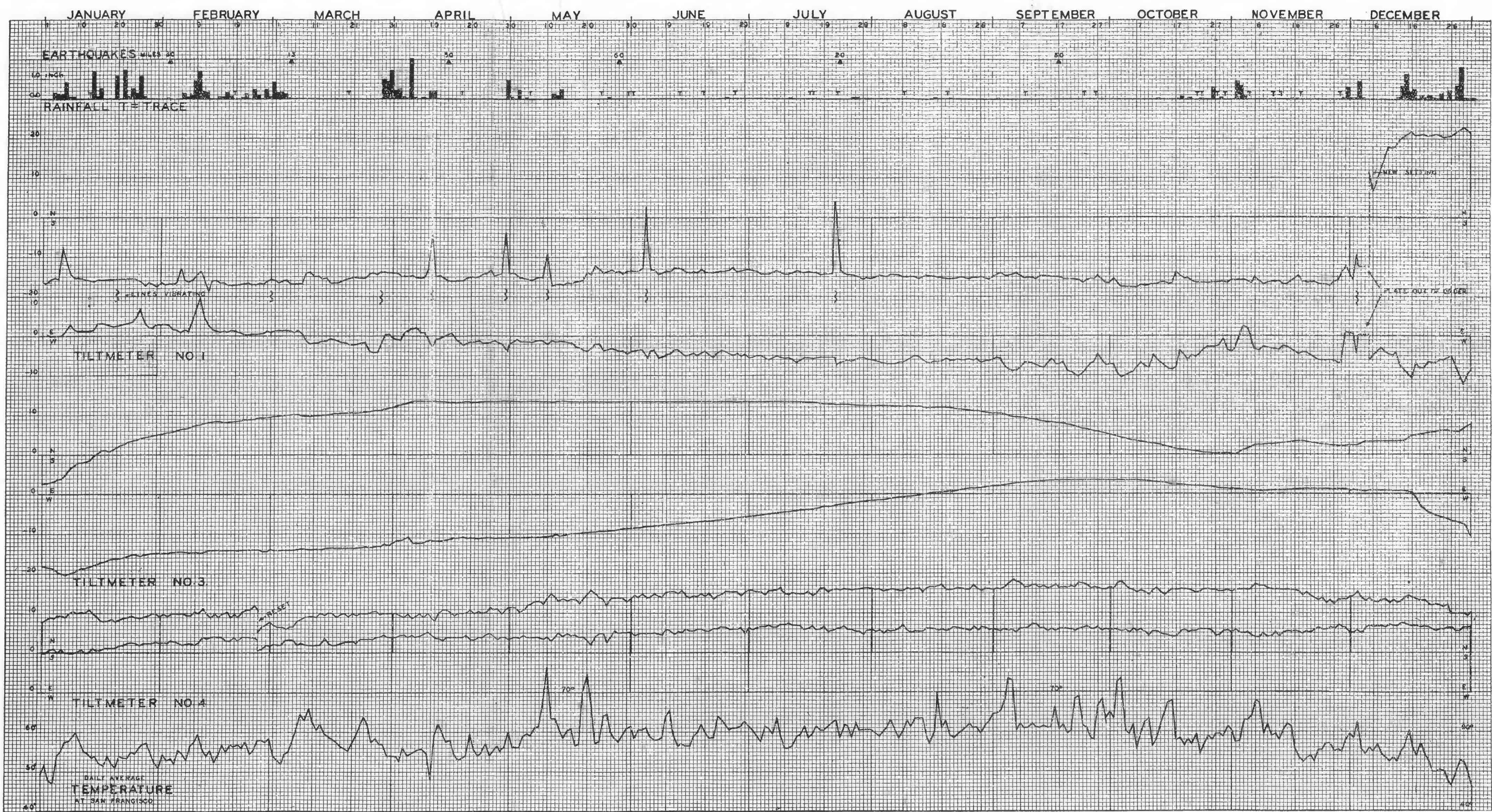
FIGURE 27.- Tilt curves for 1941.
