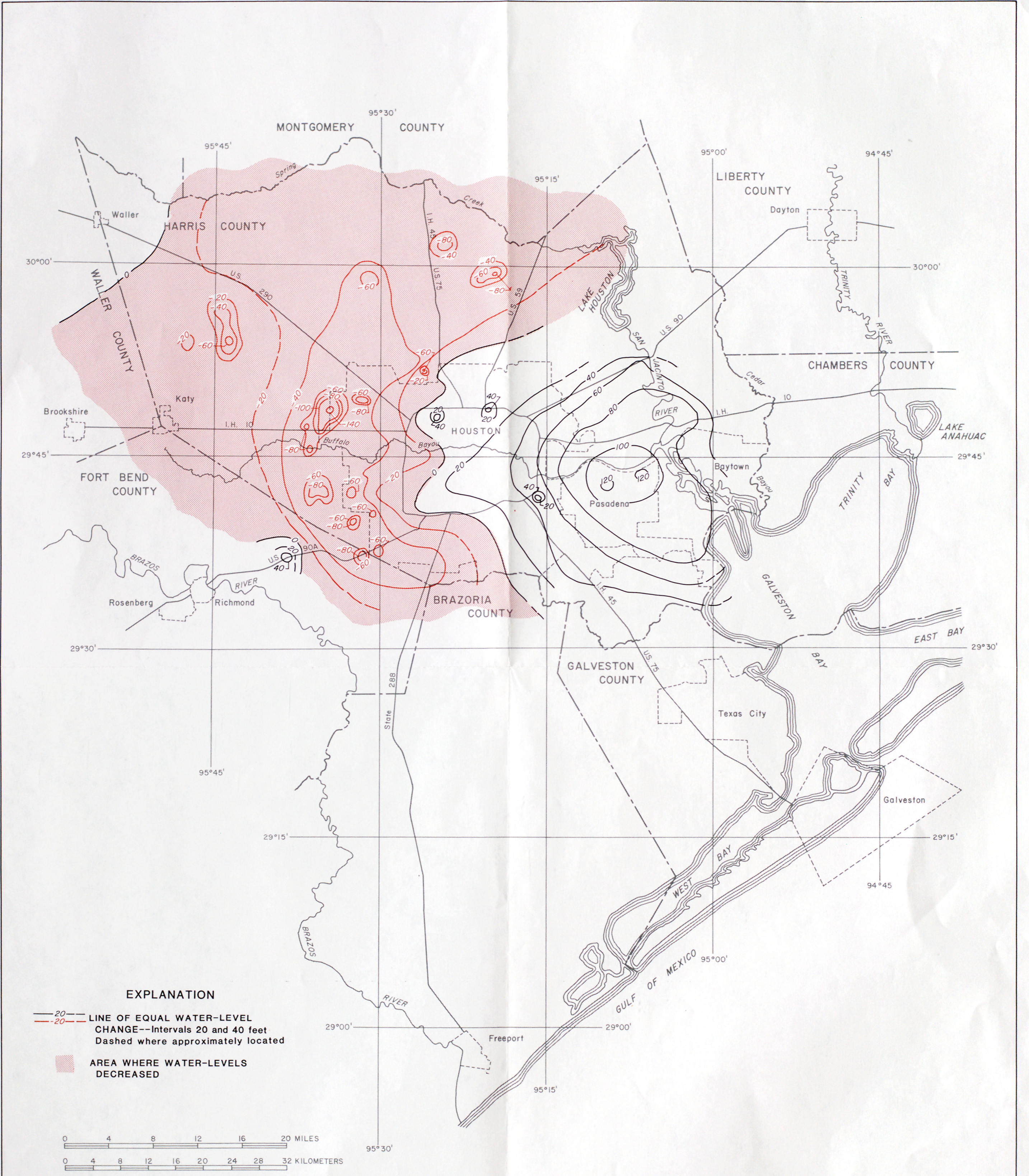
FIGURE 3.—APPROXIMATE WATER-LEVEL CHANGES IN WELLS IN THE EVANGELINE AQUIFER, 1977-85
