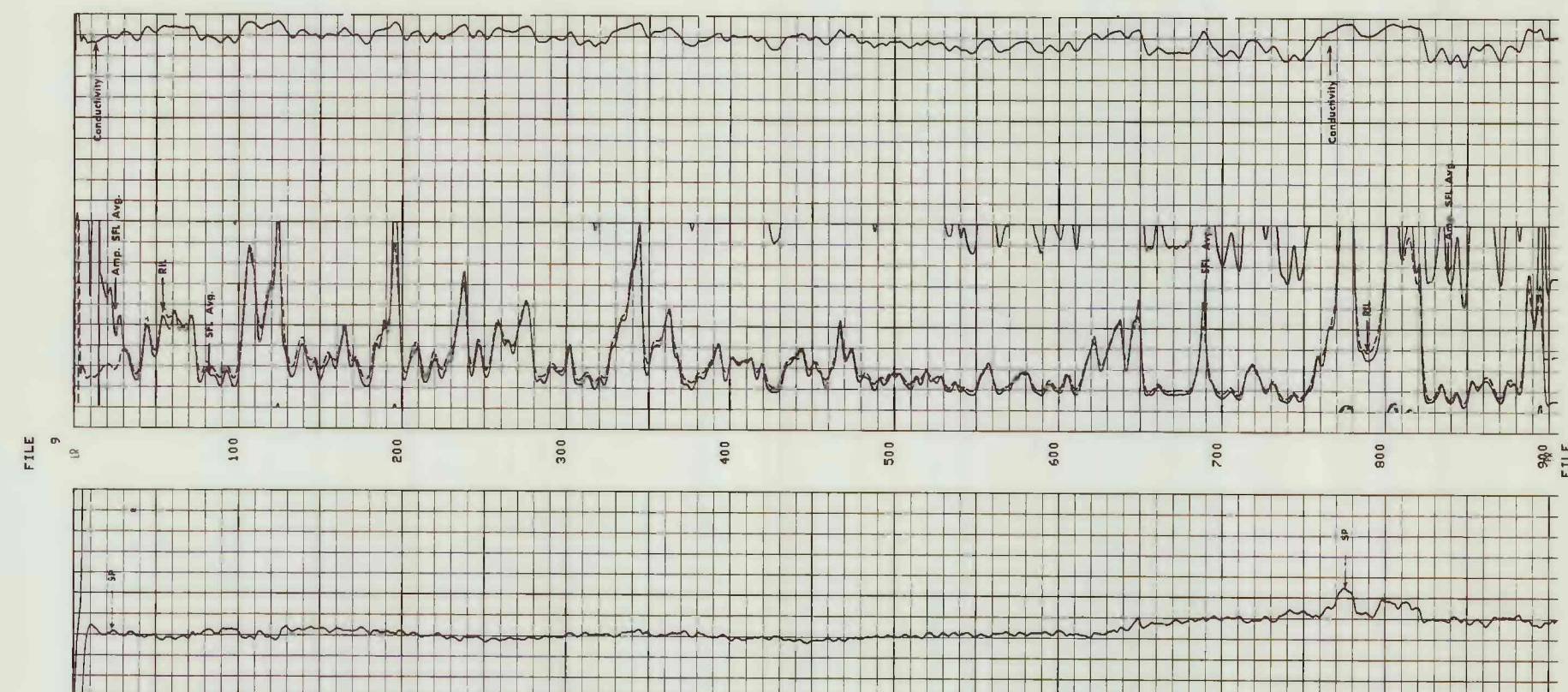
LOG A.-- Conductivity, dual induction, and spontaneous potential
