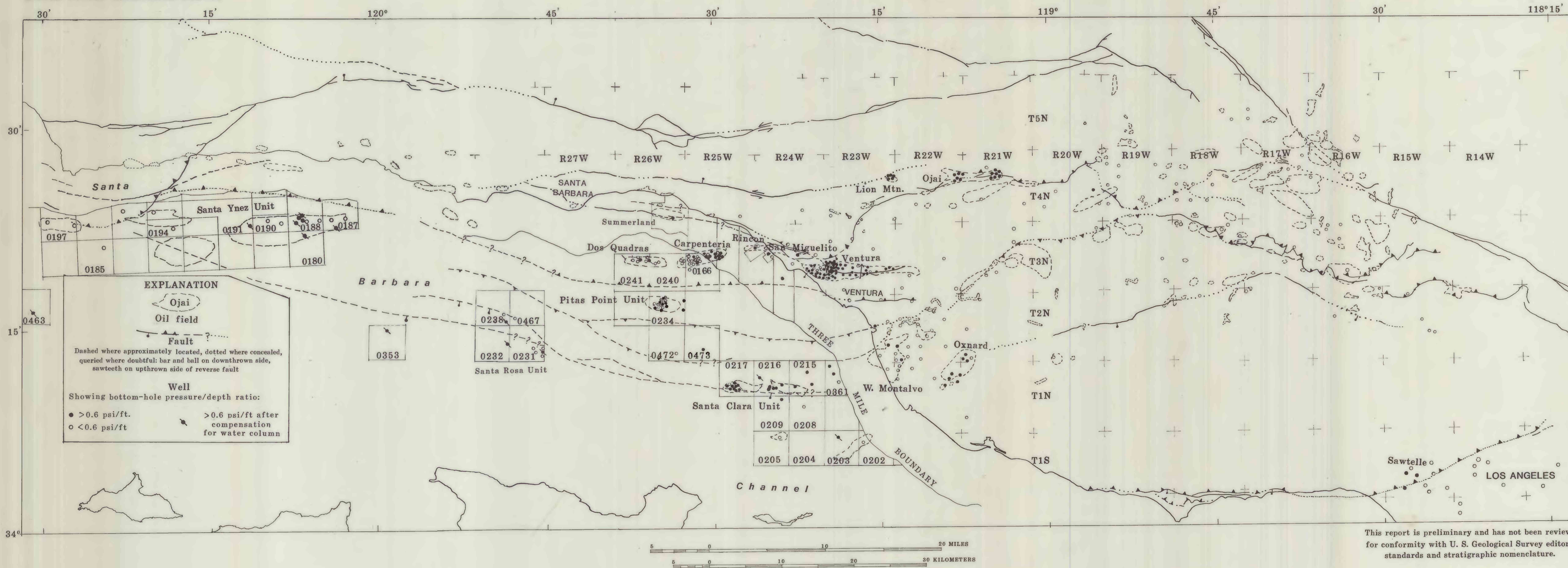
Plate 1-- MAP OF WESTERN TRANSVERSE RANGES, CALIFORNIA, SHOWING WELLS HAVING ABNORMALLY HIGH PORE PRESSURES
