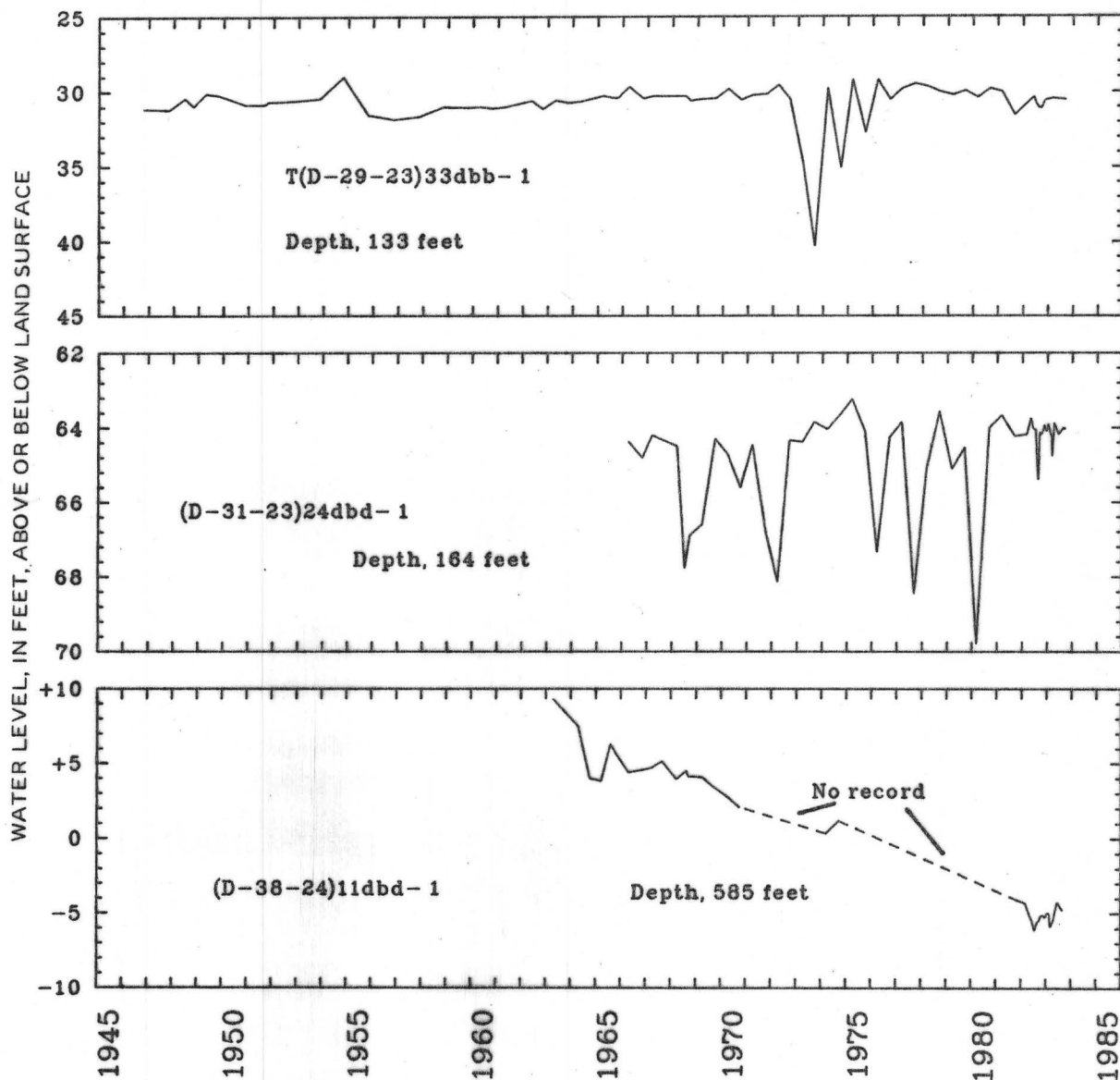
Figure 13.—Long-term water levels in three wells completed in the N aquifer.
