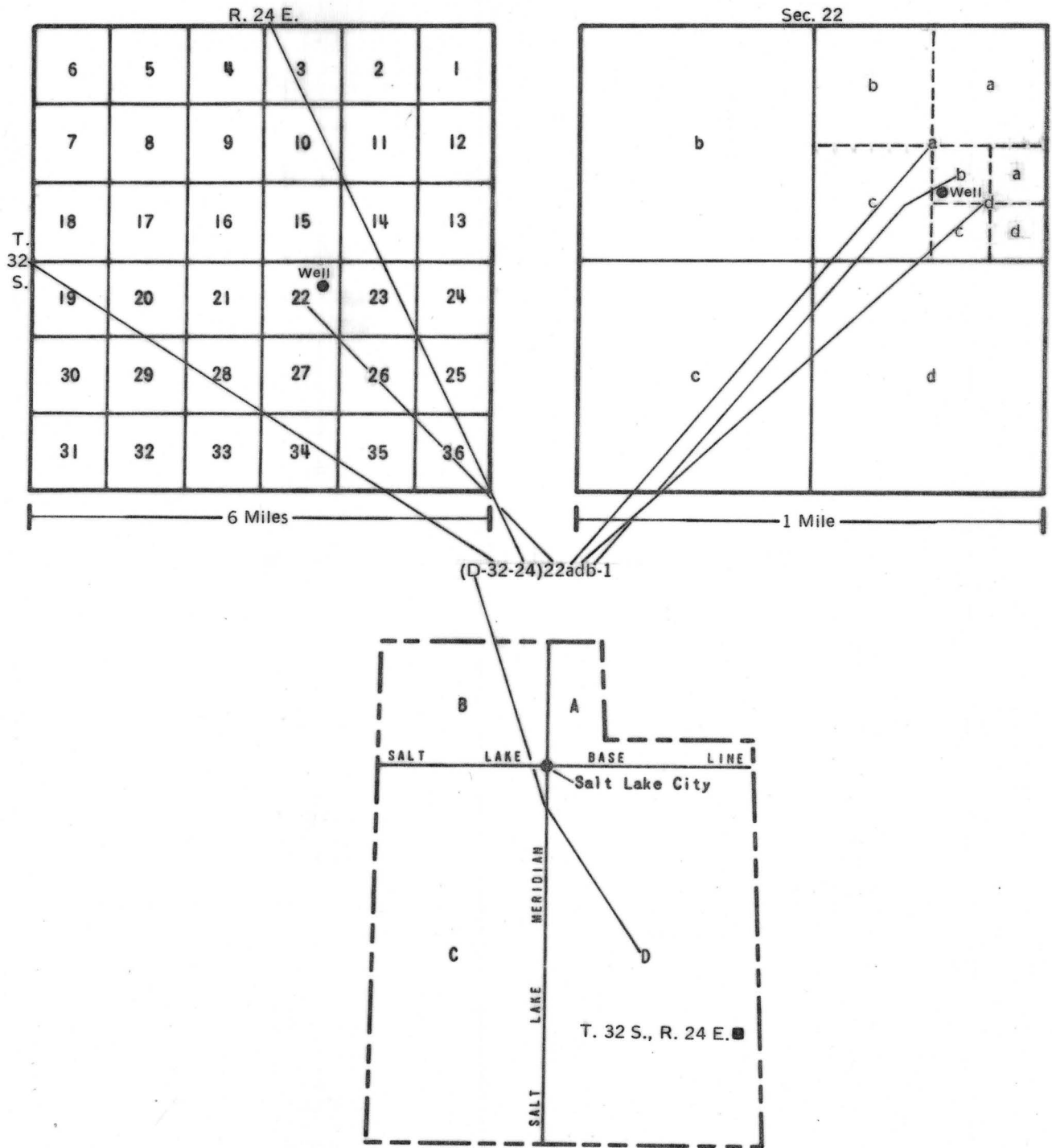
Figure 2.—Numbering system for wells and springs used in Utah.
