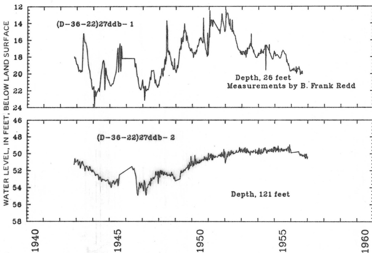
Figure 20.—Water levels in wells (D-36-22)27ddb-1 and (D-36-22)27ddb-2 completed in the D aquifer at Blanding, 1942-56.
