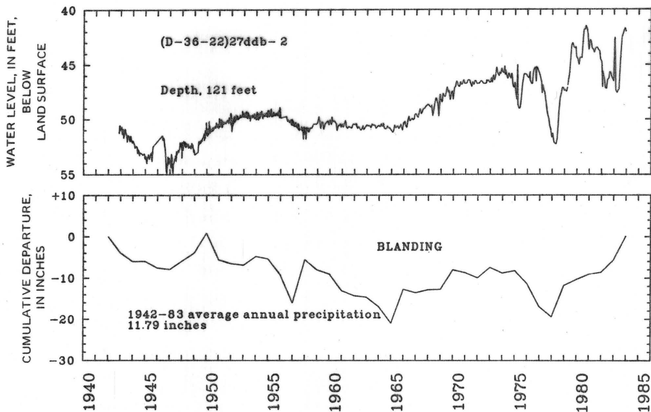
Figure 21.—Water levels in well (D-36-22)27ddb-2 completed in the D aquifer and the cumulative departure from annual precipitation at Blanding, 1942-83.
