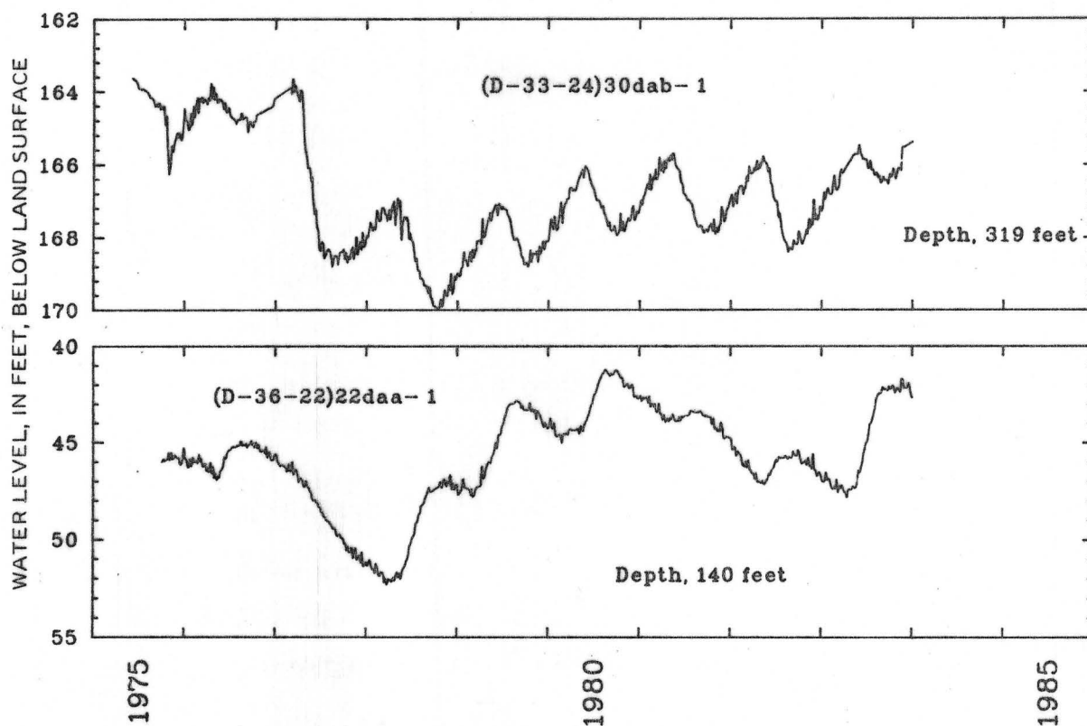
Figure 23.—Water levels from continuous automatic recorders at two wells completed in the D aquifer, 1975-83.
