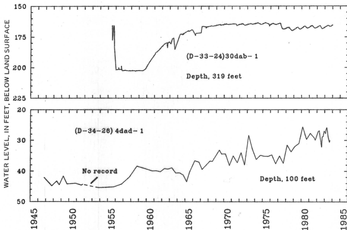
Figure 24.—Long-term water levels in two wells completed in the D aquifer near Monticello.
