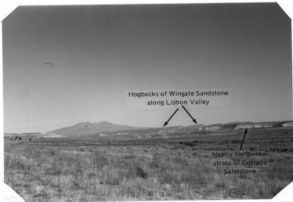
Figure 5.—View of Dry Valley, with the La Sal Mountains in the background. The hogbacks along the horizon, which are the eroded west limb of the Lisbon anticline, are a recharge area. The mountains rise from a base at an approximate altitude of 7,000 feet to Mount Peale at 12,721 feet. The vegetation consists of grassland with greasewood in the valley bottom.
