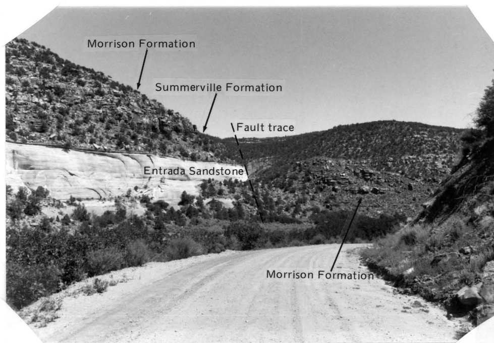
Figure 9.—View of a fault trace, which is part of the Verdure graben, present in Montezuma Creek canyon at Verdure Creek. The Morrison Formation, on the right, lies against the Entrada Sandstone, on the left, and indicates a fault displacement of about 200 feet.
