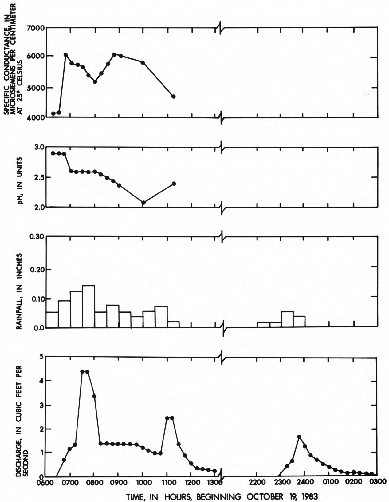
Figure 7.--Specific conductance, pH, rainfall, and discharge during storm runoff at North Fork Claybank Creek tributary near Keota (site 8), October 19 and 20, 1983.
