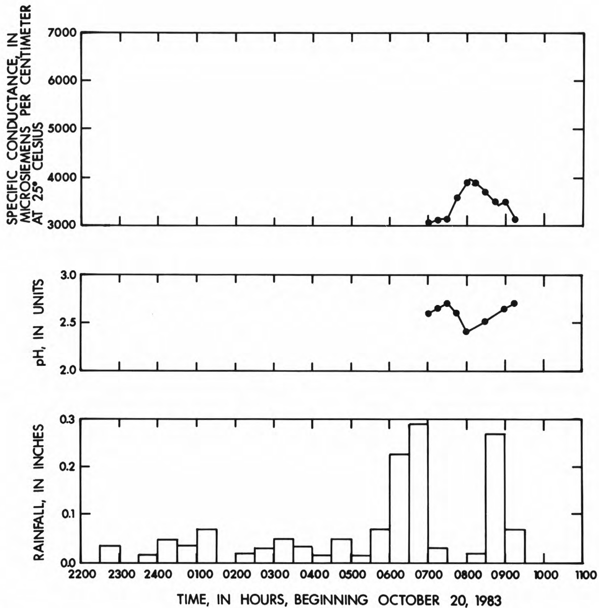
Figure 8.--Specific conductance, pH, rainfall, and discharge during storm runoff at North Fork Claybank Creek tributary near Keota (site 8) October 20 and 21, 1983--Continued
