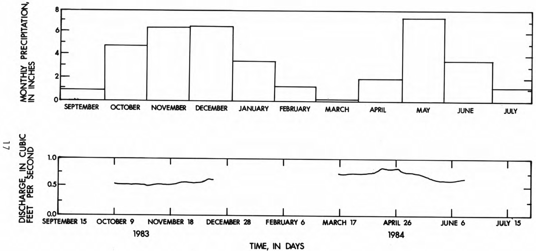
Figure 6.--Plot of ground-water levels in underground mines, continuous discharge from Mine 25 at site 18, and monthly precipitation--Continued
