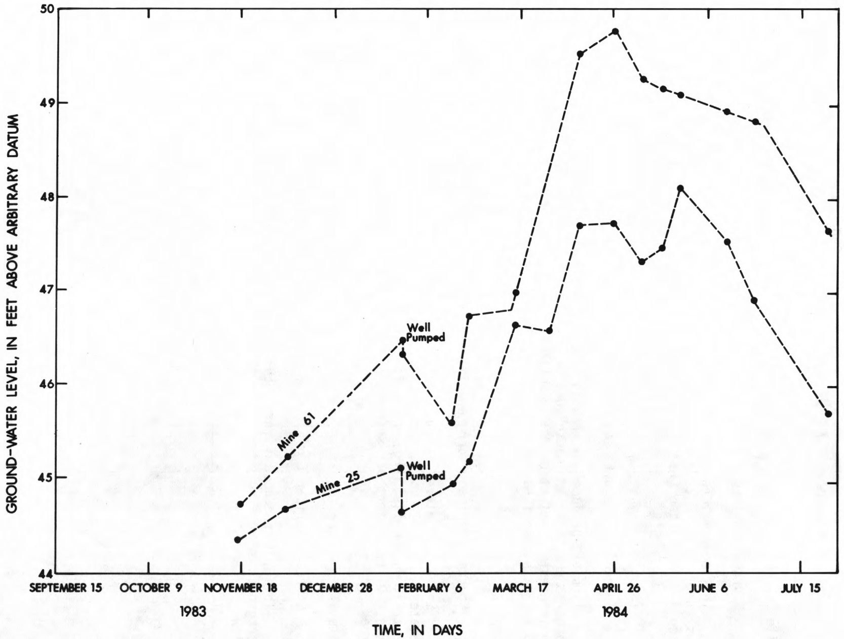
Figure 6.--Plot of ground-water levels in underground mines, continuous discharge from Mine 25 at site 18, and monthly precipitation.
