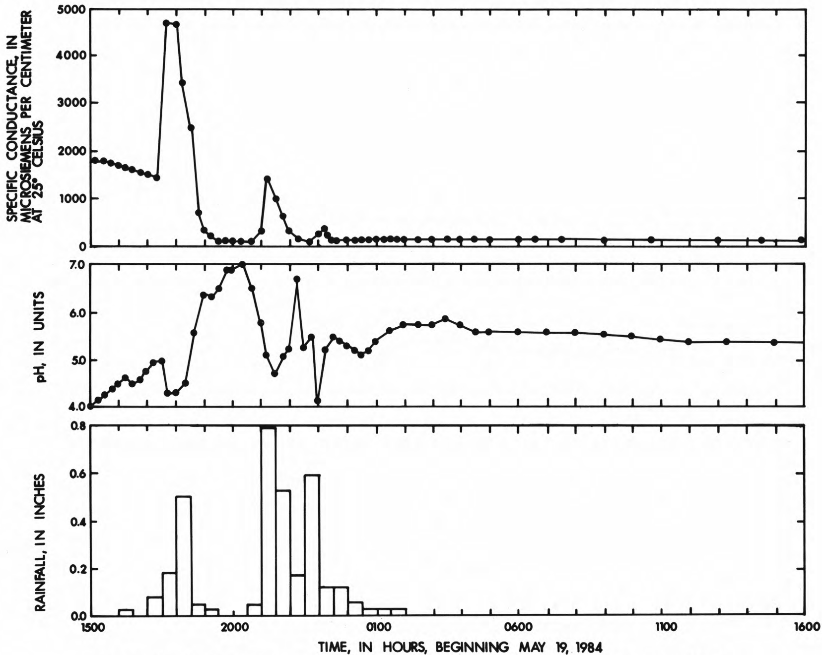
Figure 9.--Specific conductance, pH, rainfall, and stage during storm runoff at North Fork Claybank Creek tributary near Keota (site 8), May 19 and 20, 1984--Continued
