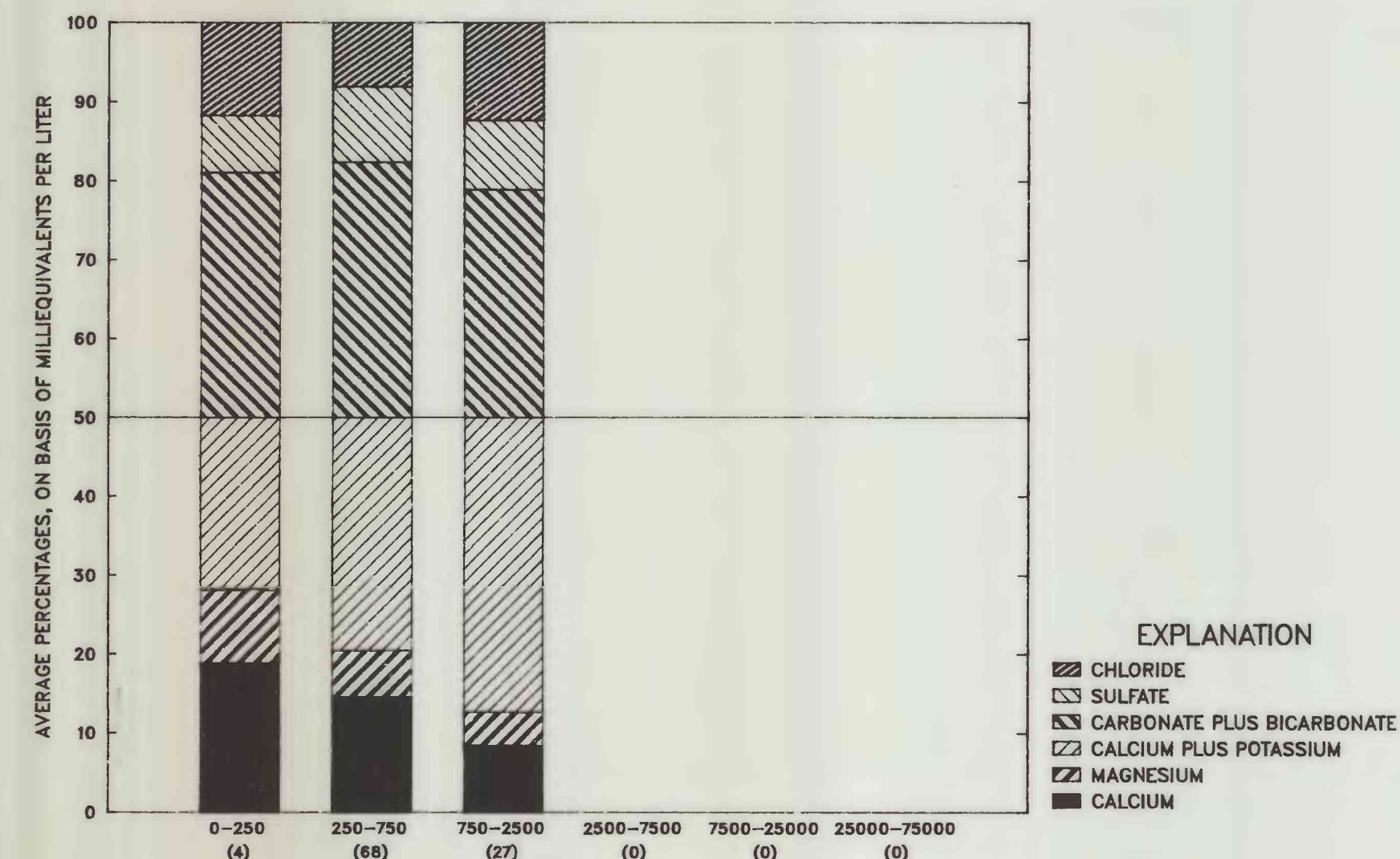
RELATION BETWEEN DISSOLVED-SOLIDS CONCENTRATION AND RELATIVE PROPORTIONS OF MAJOR IONS
