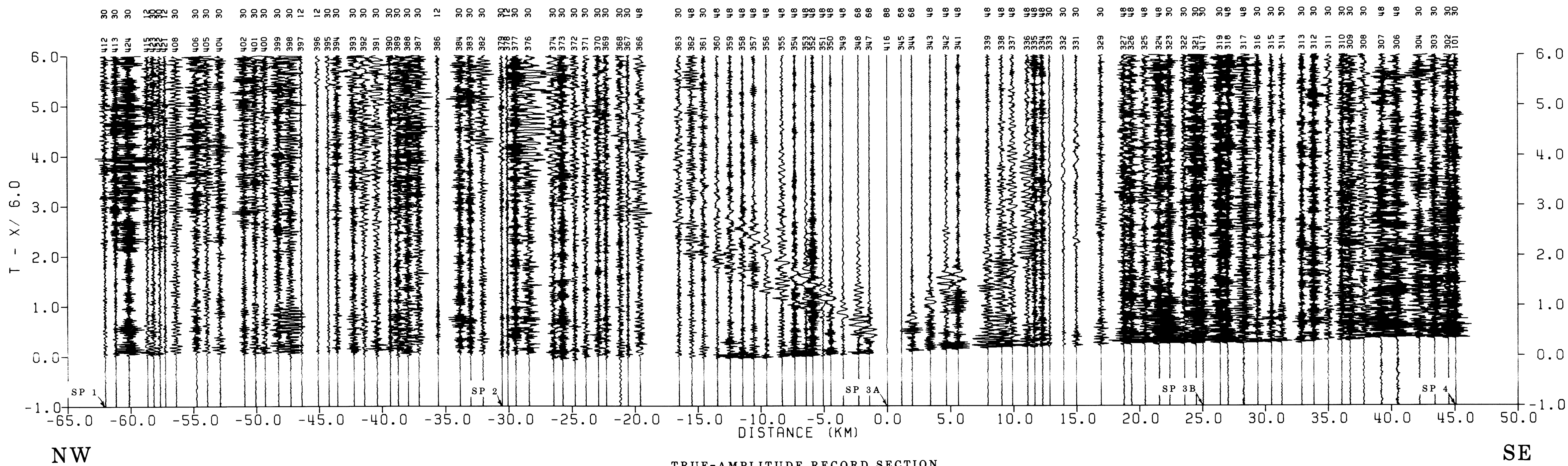
TRUE-AMPLITUDE RECORD SECTION
