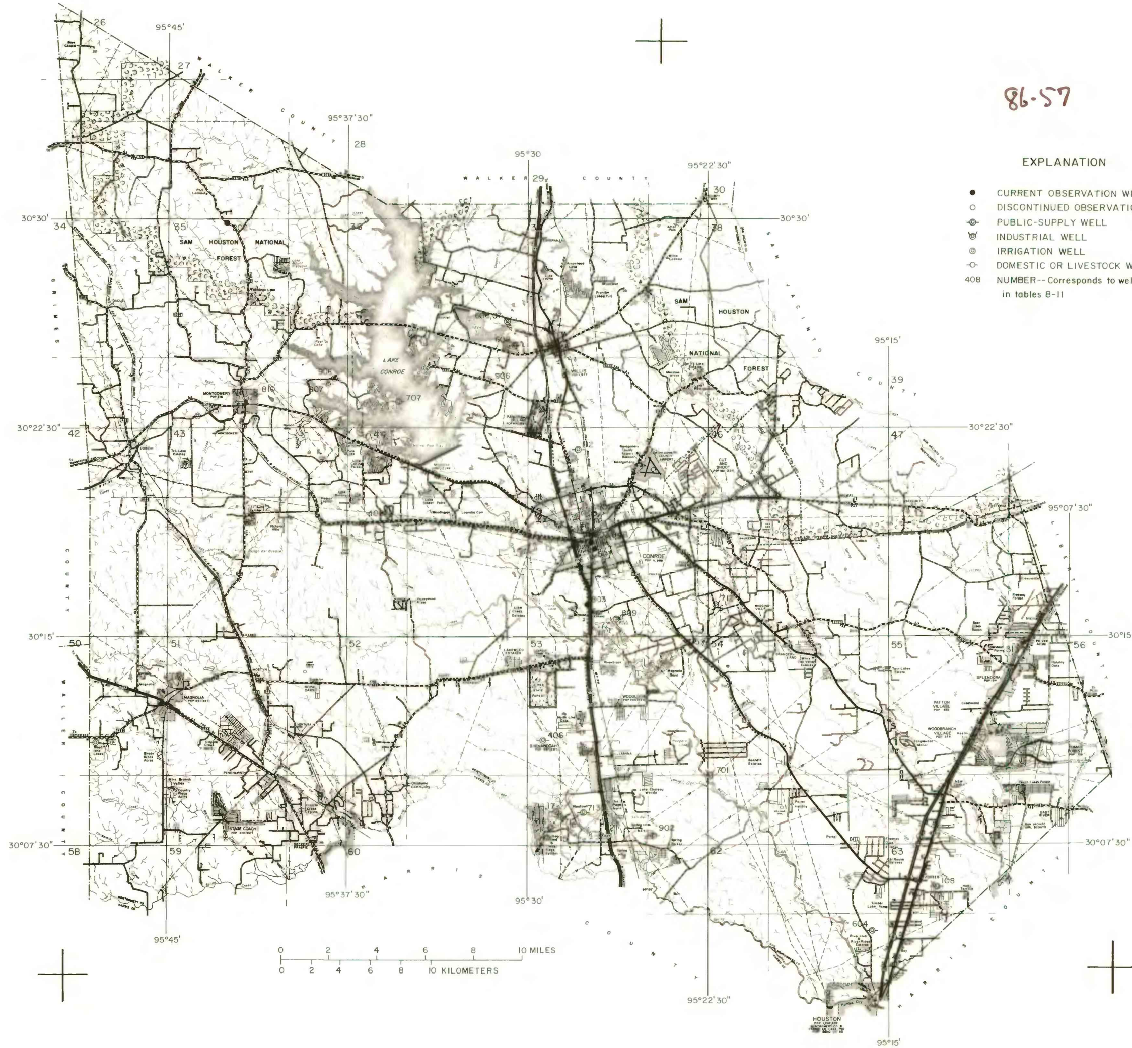
Figure 3.—Locations of wells in Montgomery County
