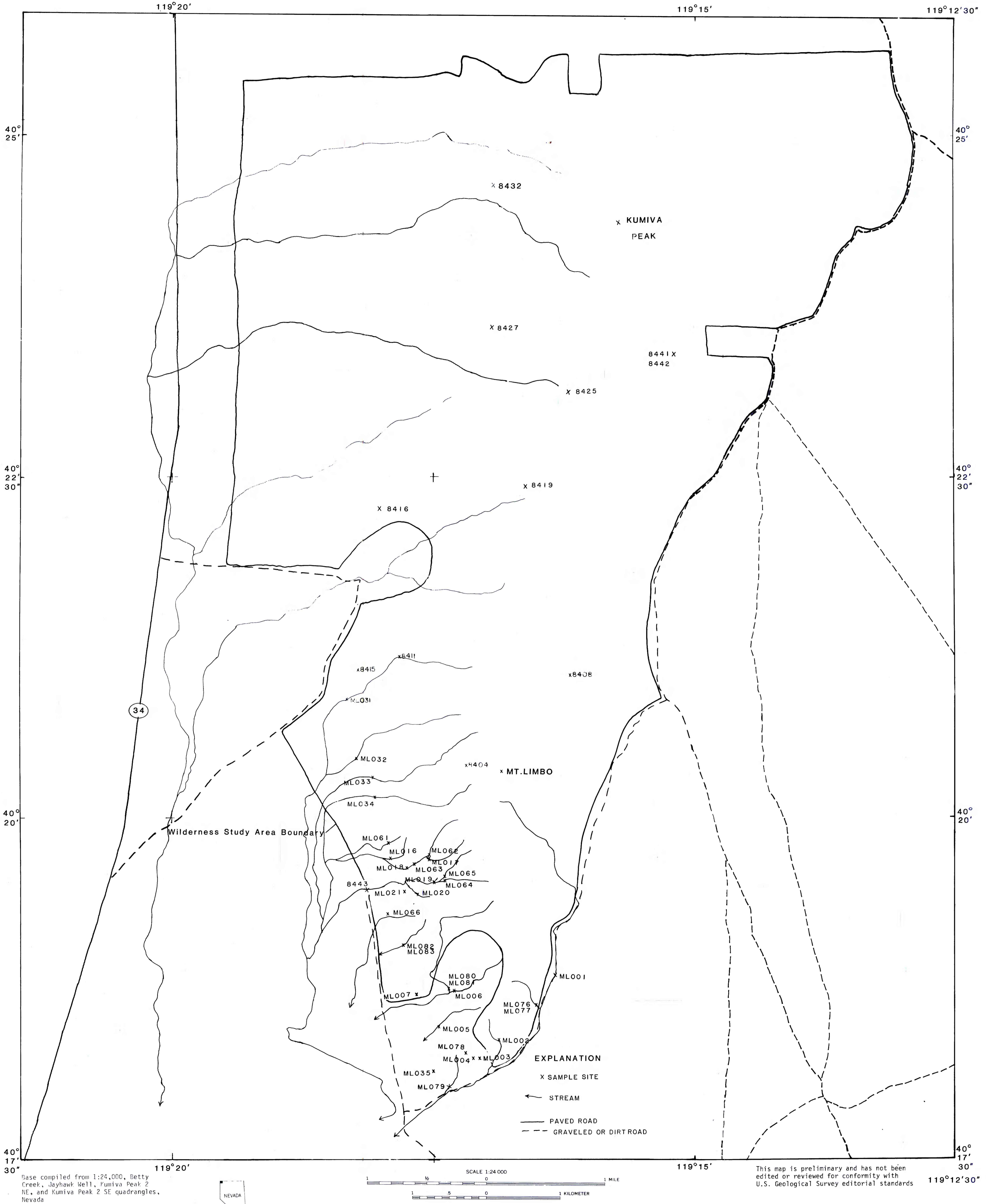
PLATE 1.-LOCALITIES OF HEAVY-MINERAL-CONCENTRATE SAMPLES, MOUNT LIMBO WILDERNESS (NV-020-201), PERSHING COUNTY, NEVADA
