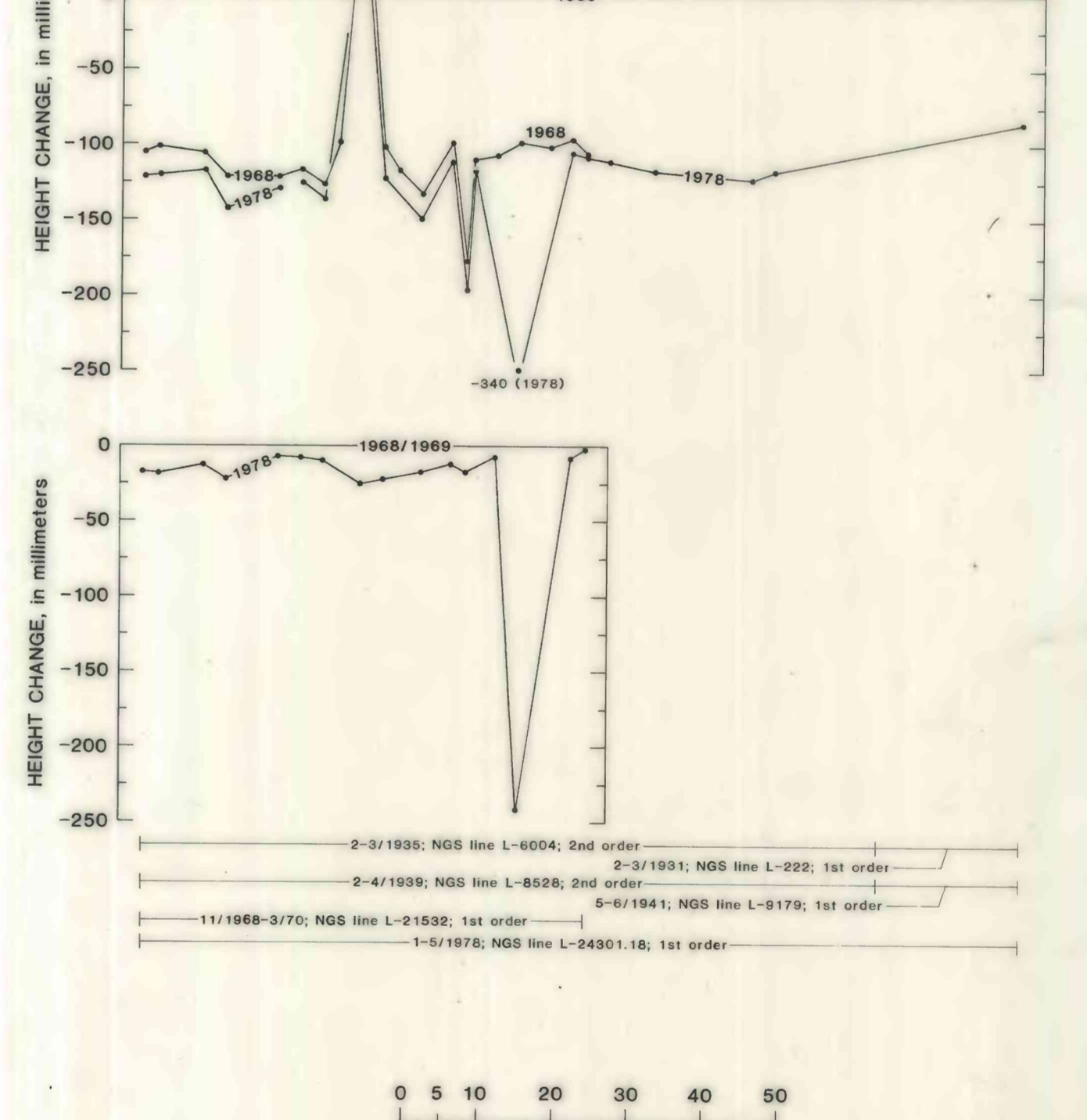
PROFILES SHOWING TERRAIN AND HEIGHT CHANGES ALONG SEVERAL ROUTES BETWEEN SANTA YSABEL AND THE SALTON TROUGH, WITH RESPECT TO BENCH MARK M57, SAN DIEGO
