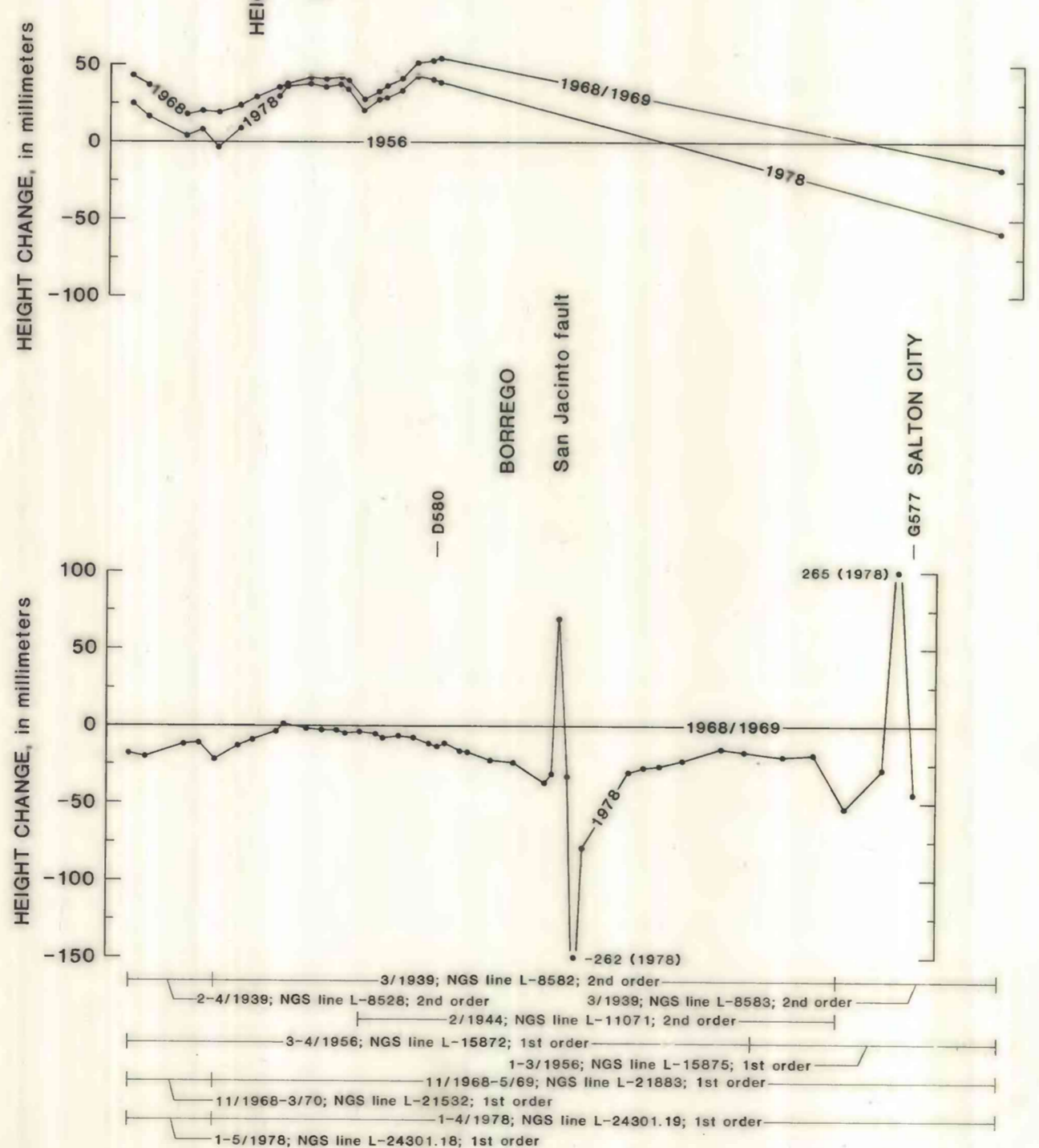
PROFILES SHOWING TERRAIN AND HEIGHT CHANGES ALONG SEVERAL ROUTES BETWEEN SANTA YSABEL AND THE SALTON TROUGH, WITH RESPECT TO BENCH MARK M57, SAN DIEGO
