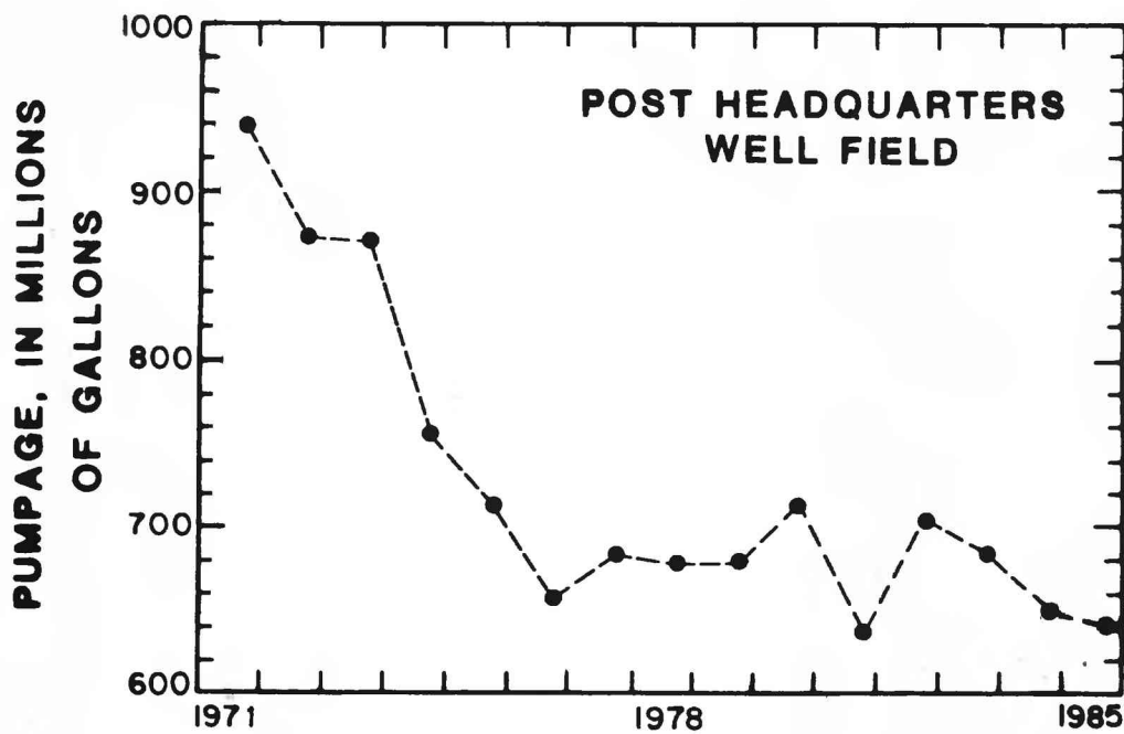
Figure 5.--Water levels in test well T-8 and yearly pumpage from the Post Headquarters well field, 1971-85.
