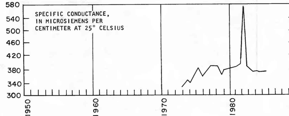
Figure 6.--Water levels and specific conductance for period of record available in selected supply wells - Continued.
