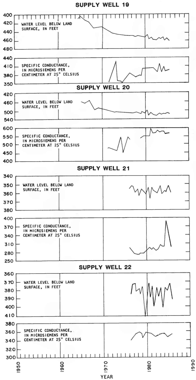
Figure 6.--Water levels and specific conductance for period of record available in selected supply wells - Concluded.
