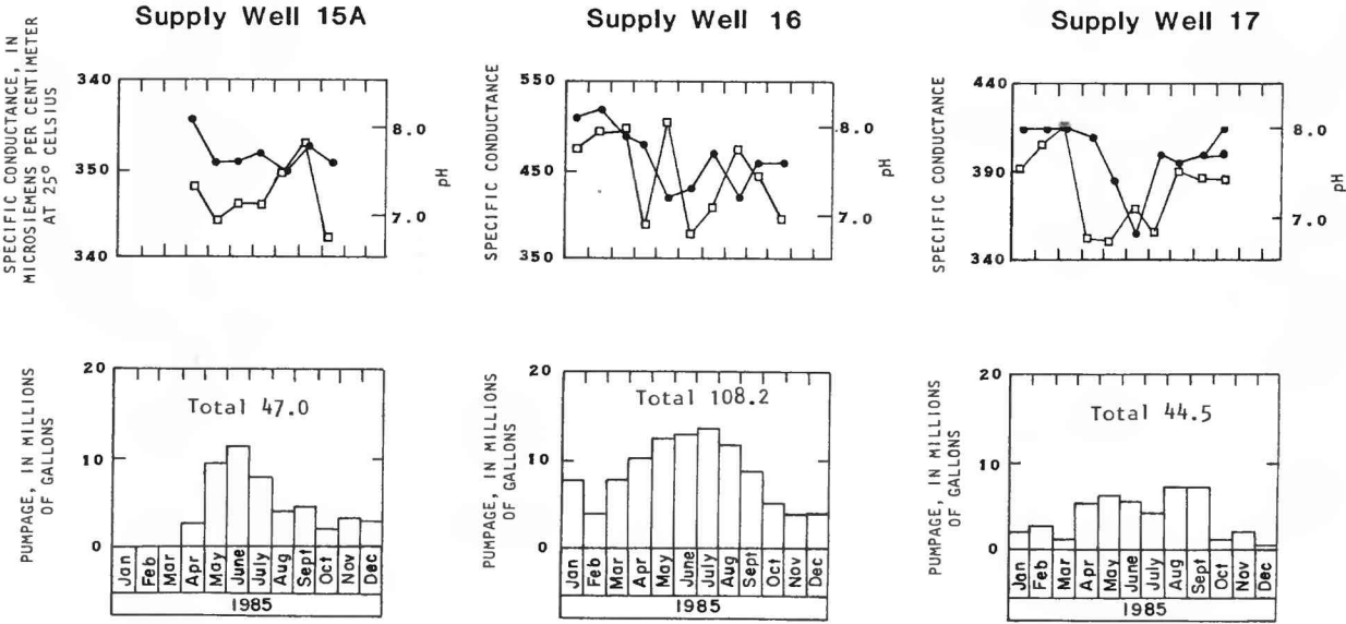
Figure 8.--Monthly specific conductance, pH, and pumpage for Post Headquarters supply wells.
