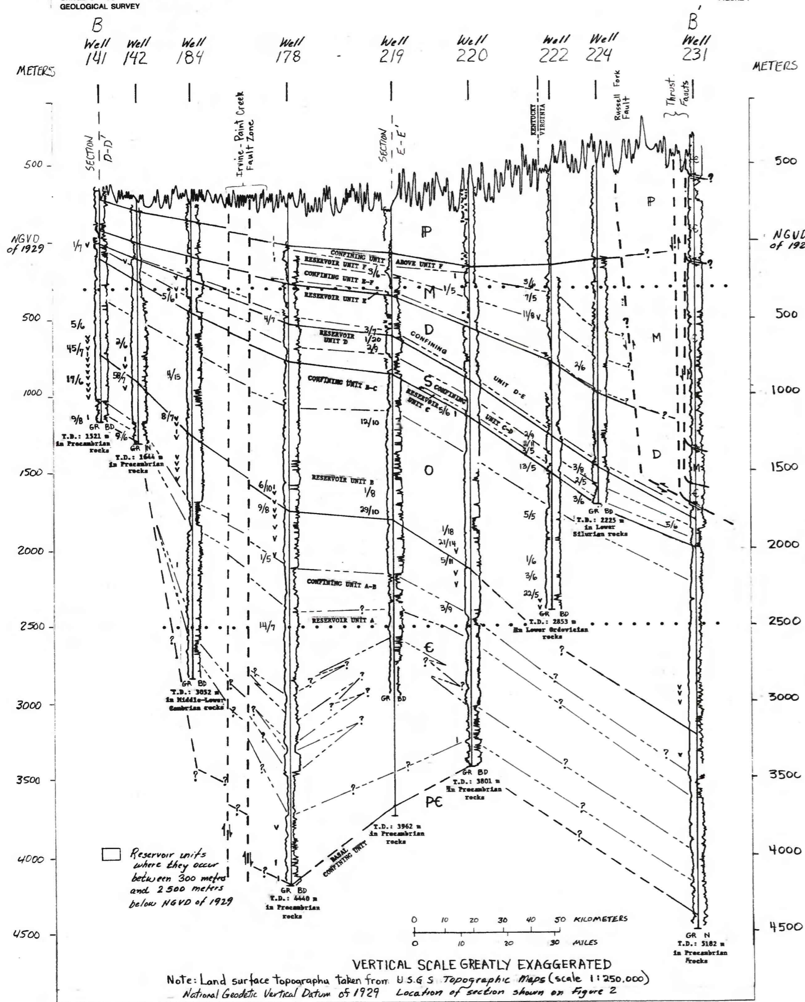
Figure 7.--Generalized geologic cross section B-B' from Rowan County, Kentucky, to Russell County, Virginia
