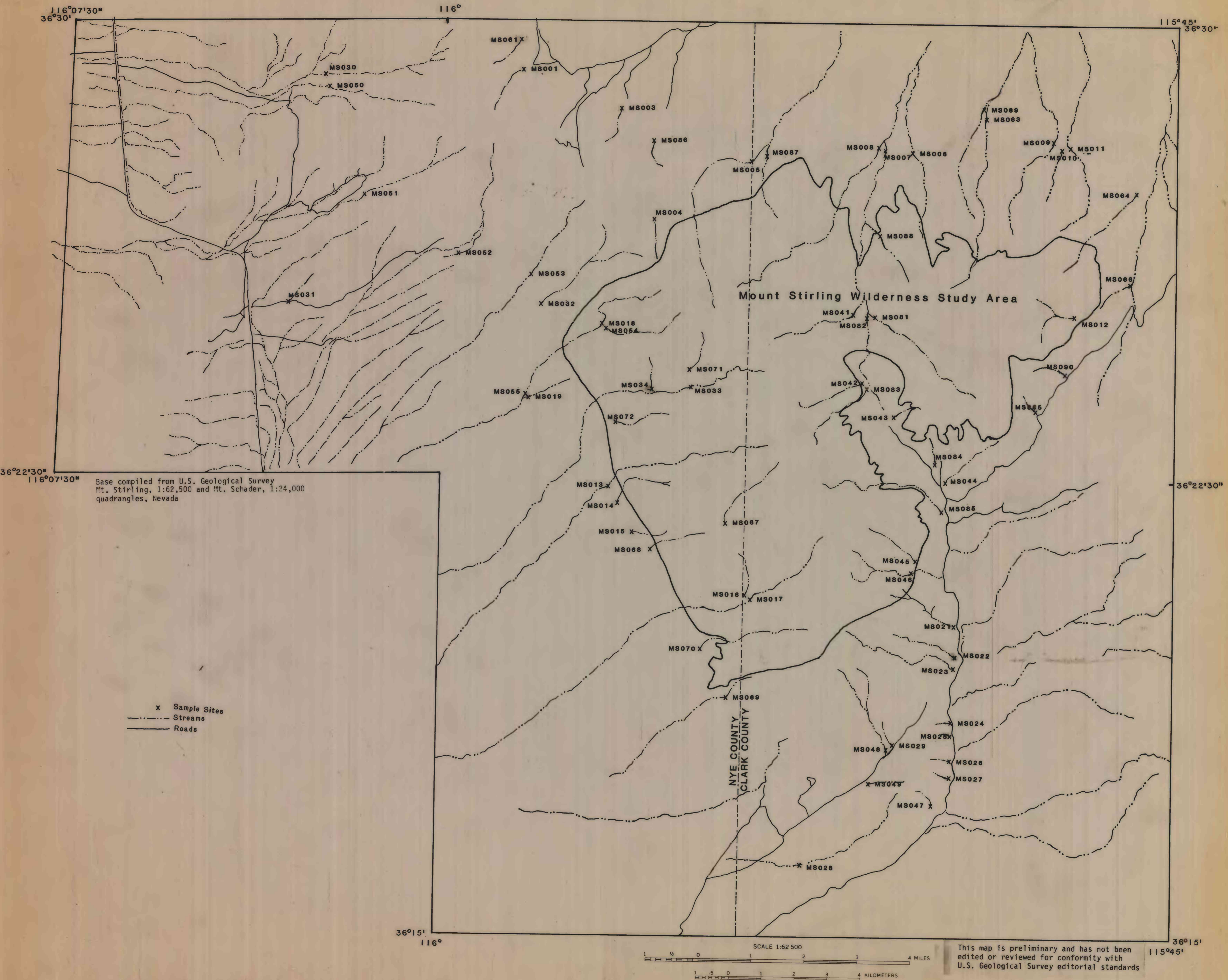
PLATE 1.-LOCALITIES OF HEAVY-MINERAL-CONCENTRATE AND ROCK SAMPLES, MOUNT STIRLING WILDERNESS STUDY AREA (NV-050-401), NYE AND CLARK COUNTIES, NEVADA
