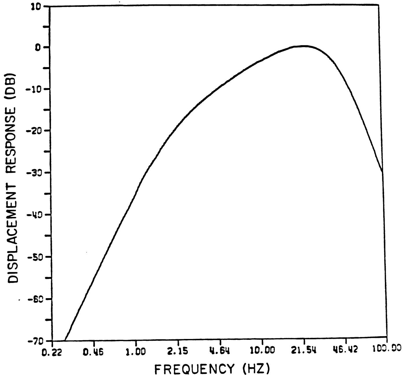
Figure 18: System response curve for cassette recording units with 2-Hz seismometers
