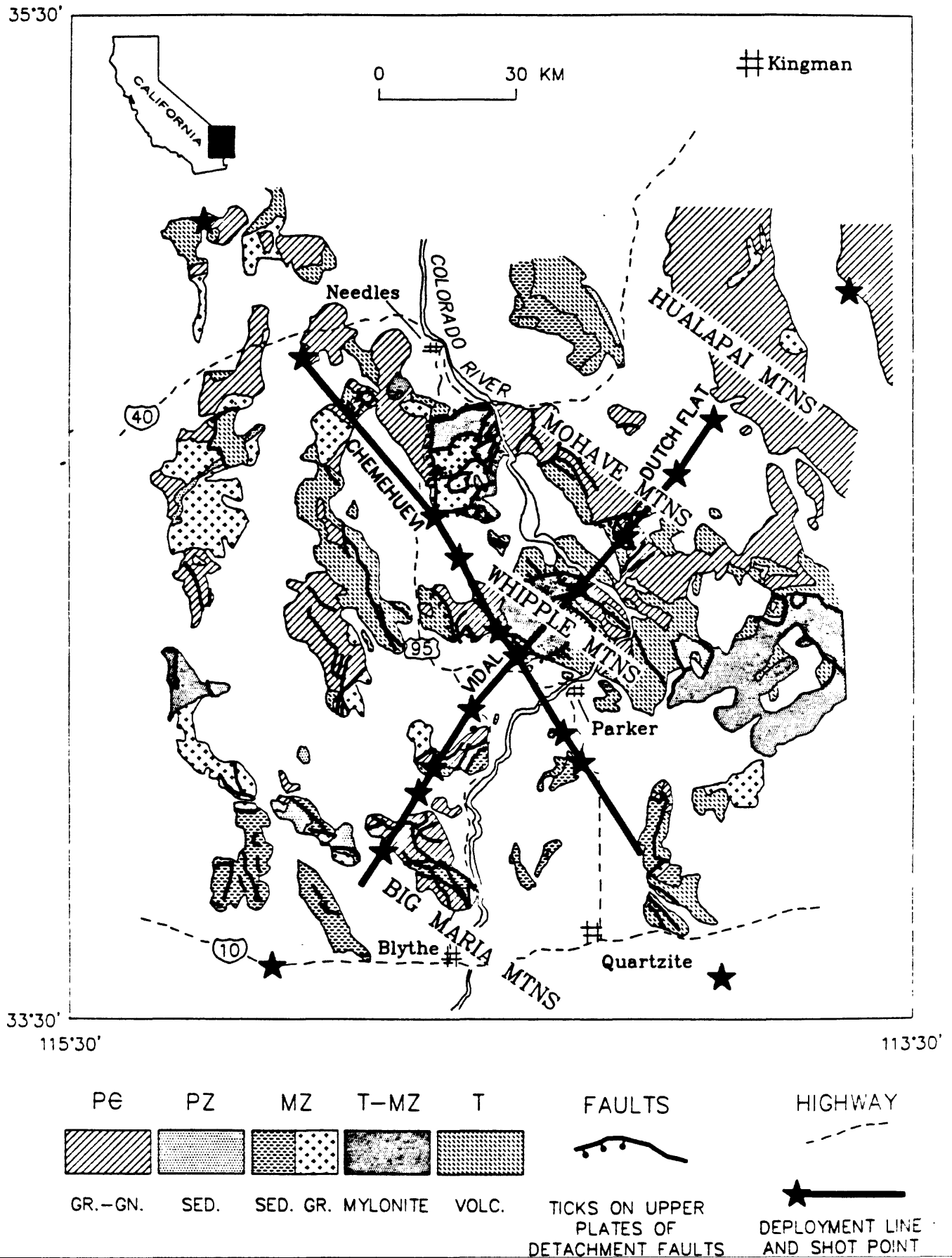
Figure 1: Geologic Map of Study Area, Compiled from Howard (1986), Jennings (1977), Reynolds (1980), and Wilson (1969).
