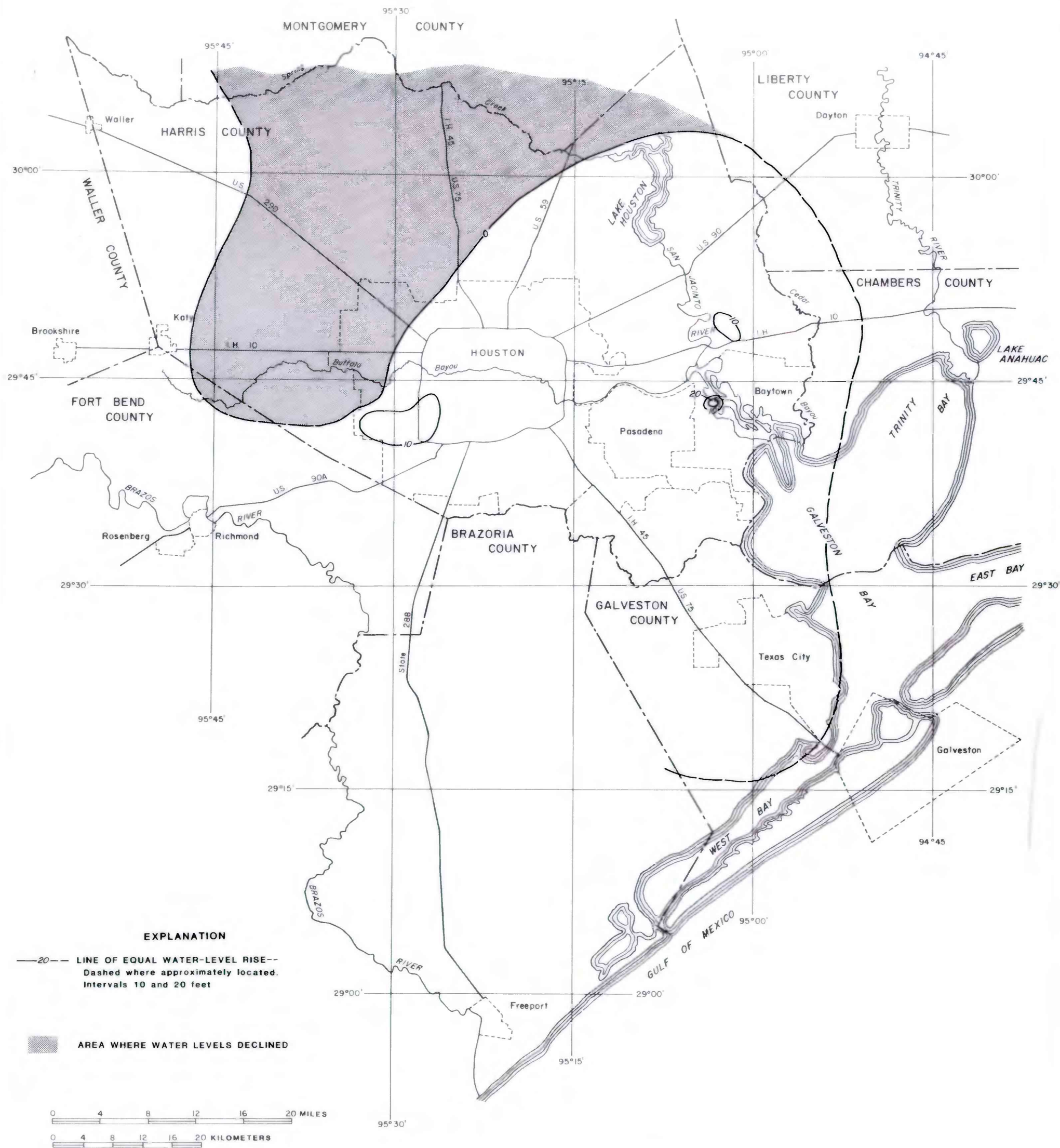
FIGURE 2.—MAP SHOWING APPROXIMATE CHANGE IN WATER LEVELS IN WELLS IN THE CHICOT AQUIFER, SPRING 1986 TO SPRING 1987.
