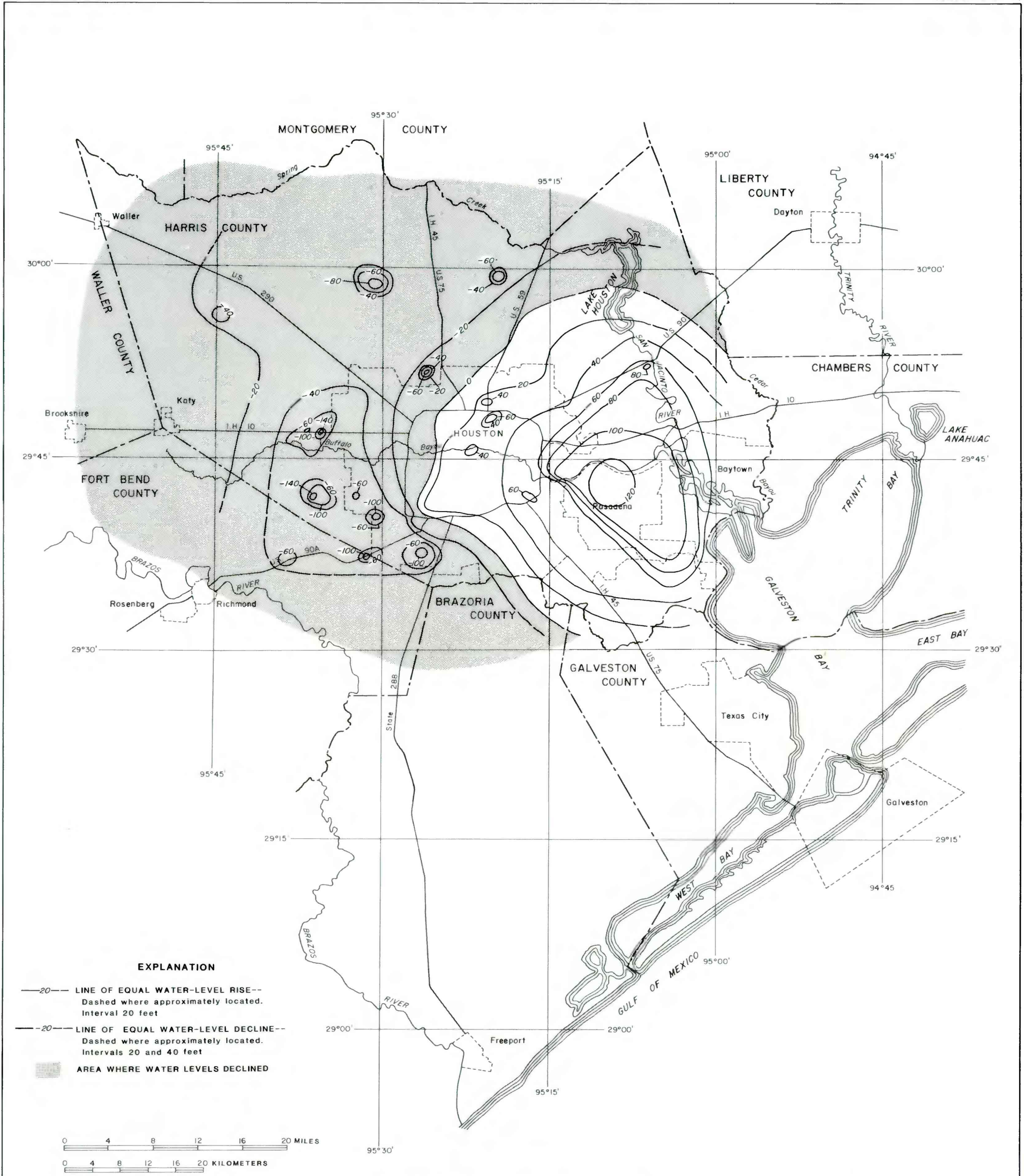
FIGURE 3.--MAP SHOWING APPROXIMATE CHANGE IN WATER LEVELS IN WELLS IN THE EVANGELINE AQUIFER, SPRING 1977 TO SPRING 1987.
