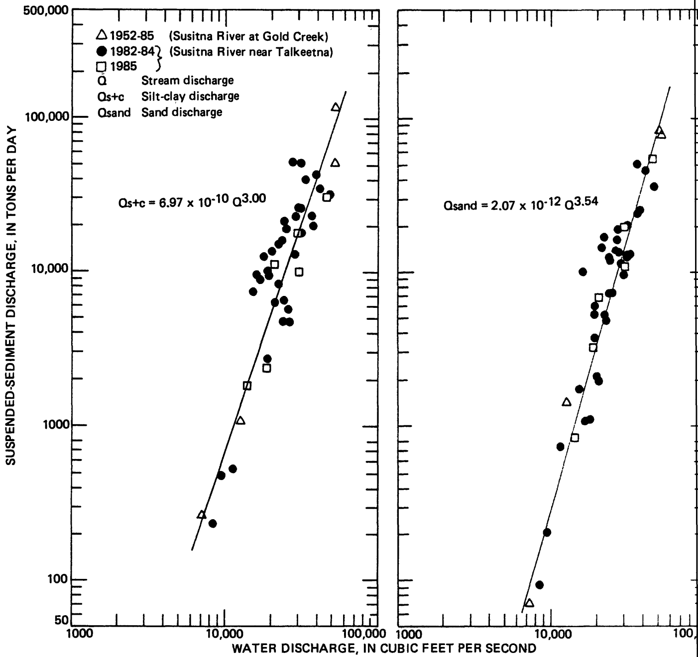
Figure 2.--Sediment-transport curves of suspended silt-clay and sand discharge for Susitna River near Talkeetna, May to September, 1981-85.
