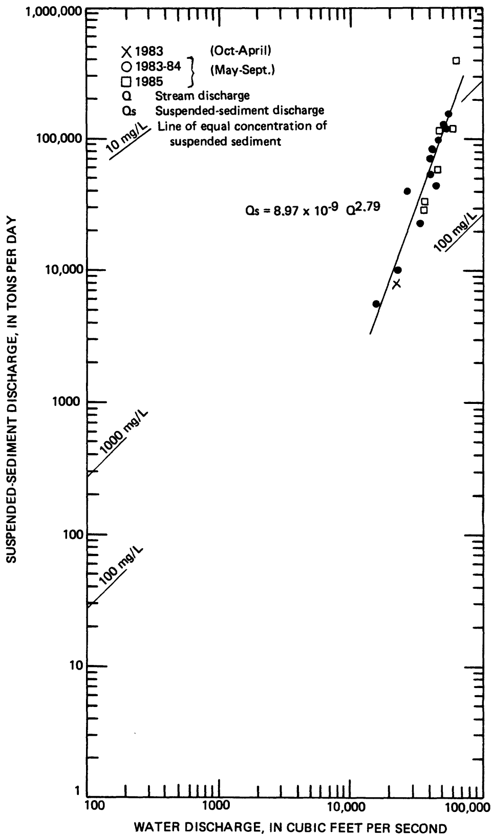
Figure 11.--Relation of mean suspended-sediment concentration and discharge to water discharge for Susitna River below Chulitna River near Talkeetna (sum of right and left channels), May to September, 1983-85.
