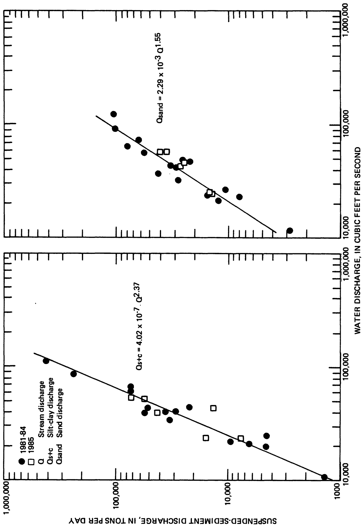
Figure 7.--Sediment-transport curves of suspended silt-clay and sand discharge for Yentna River near Susitna Station, May to September, 1981-85.
