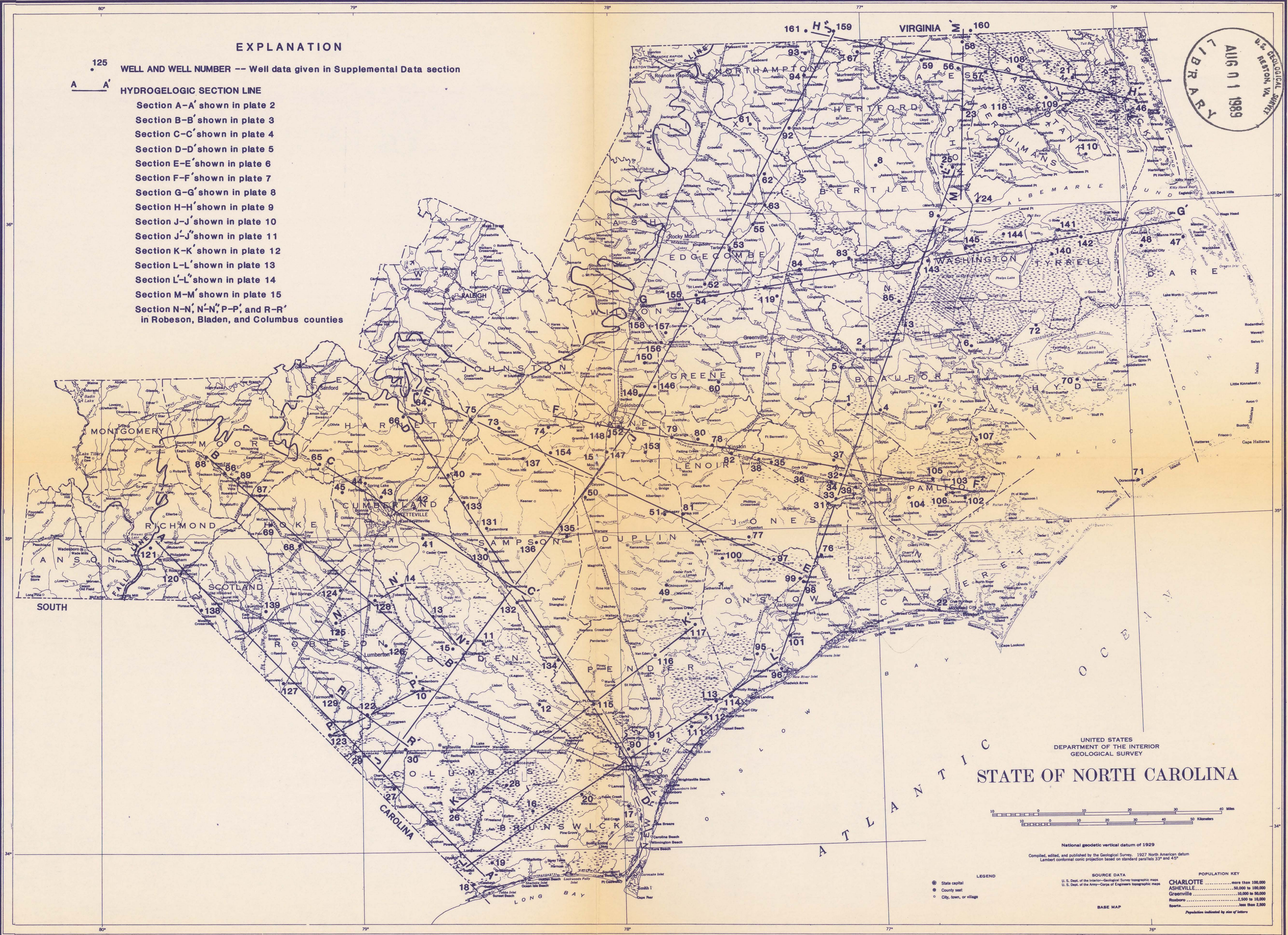
LOCATION OF WELLS AND HYDROGEOLOGIC SECTIONS
