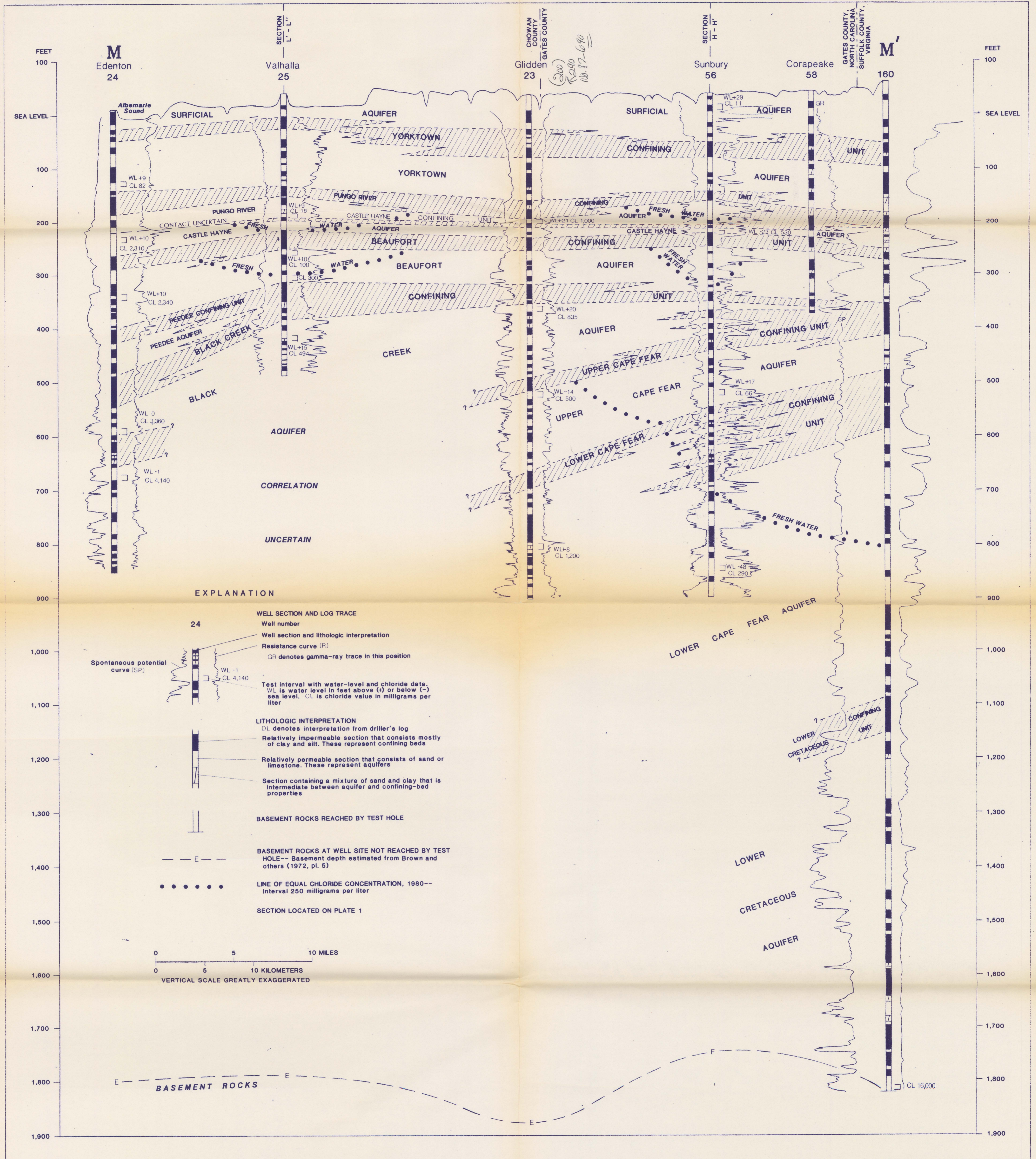
HYDROGEOLOGIC SECTION M - M' FROM EDENTON, CHOWAN COUNTY, NORTH CAROLINA TO WELL 160, SUFFOLK COUNTY, VIRGINIA.
