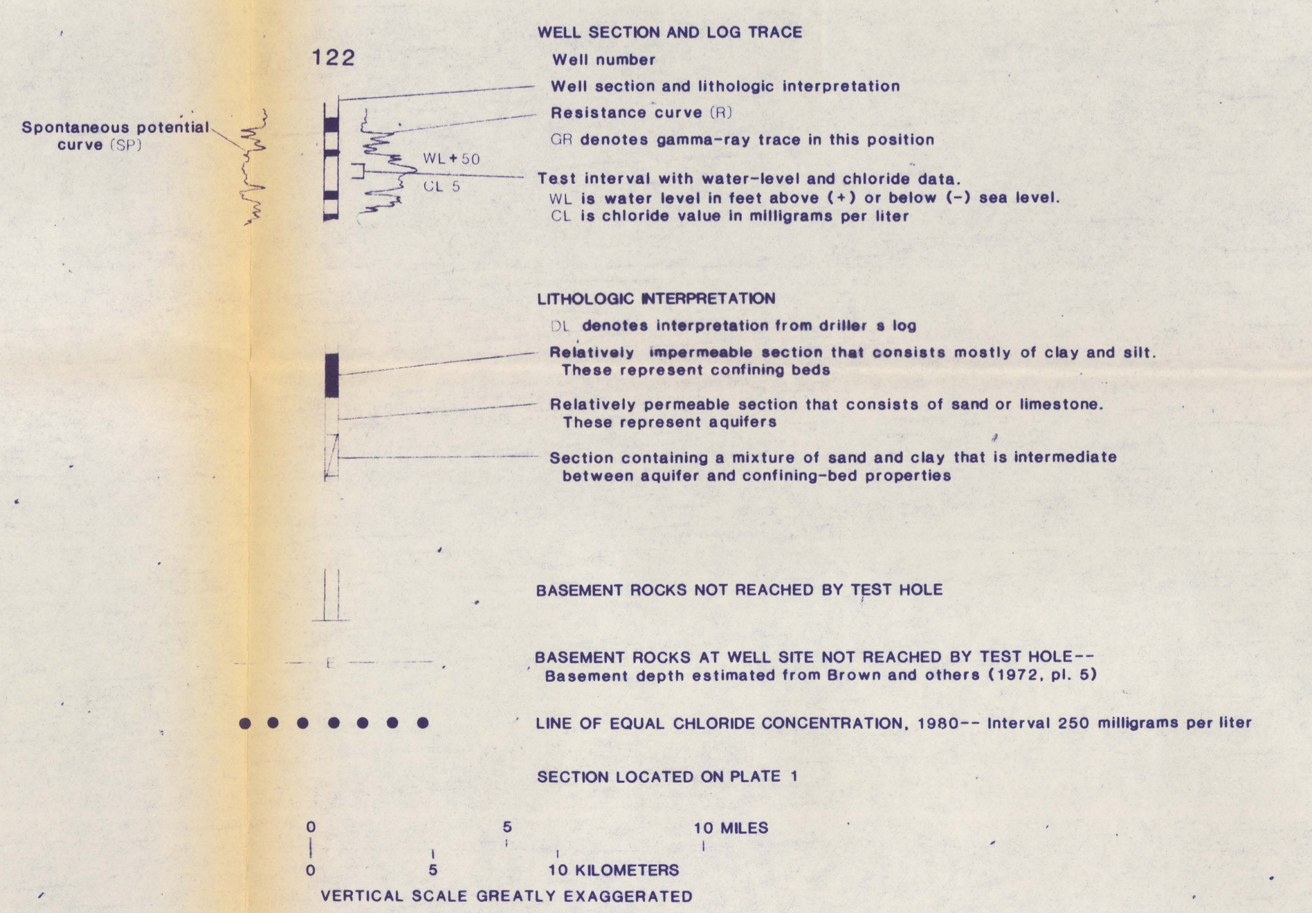
HYDROGEOLOGIC SECTIONS N-N', N'-N'', P-P', AND R-R' IN ROBESON, BLADEN, AND COLUMBUS COUNTIES
