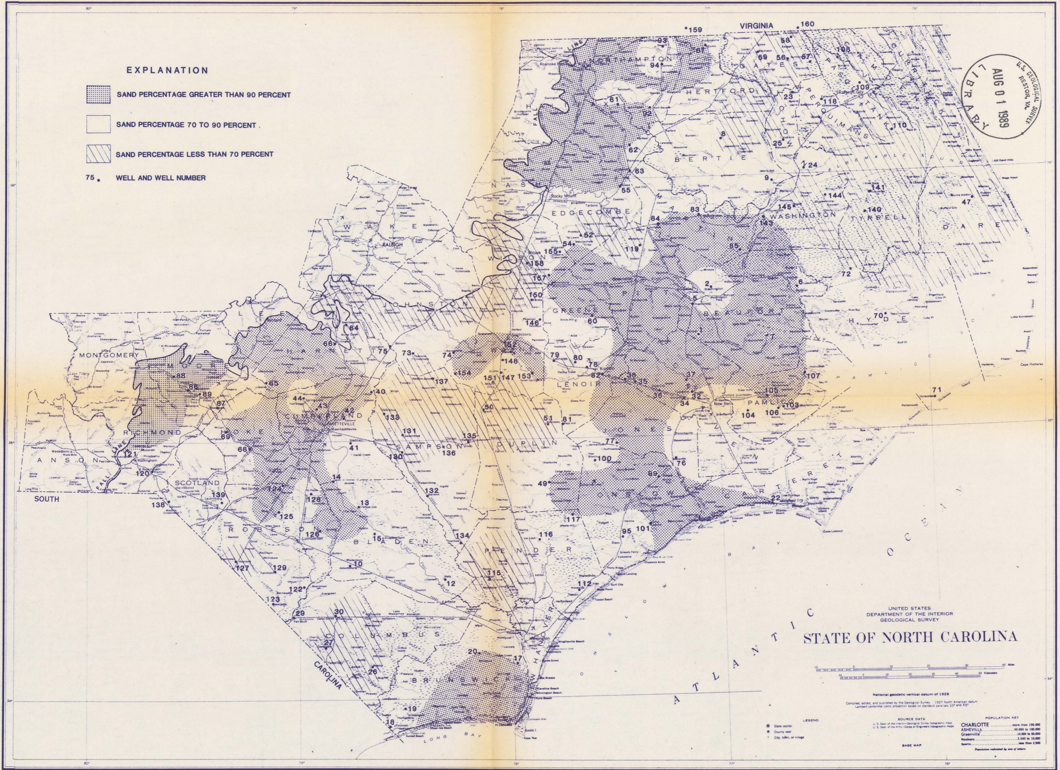
SAND PERCENTAGE IN THE SURFICIAL AQUIFER
