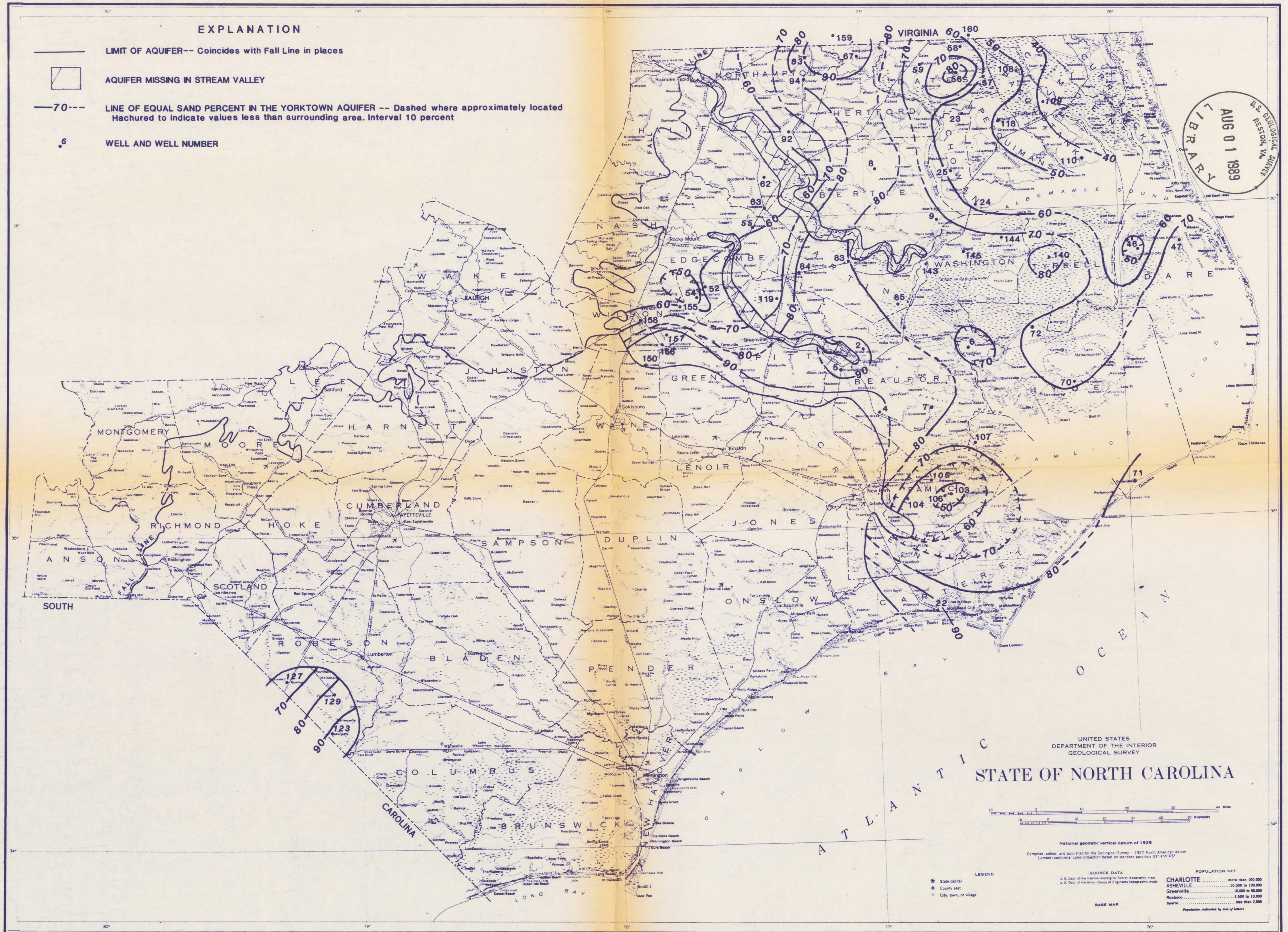
SAND PERCENTAGE IN THE YORKTOWN AQUIFER
