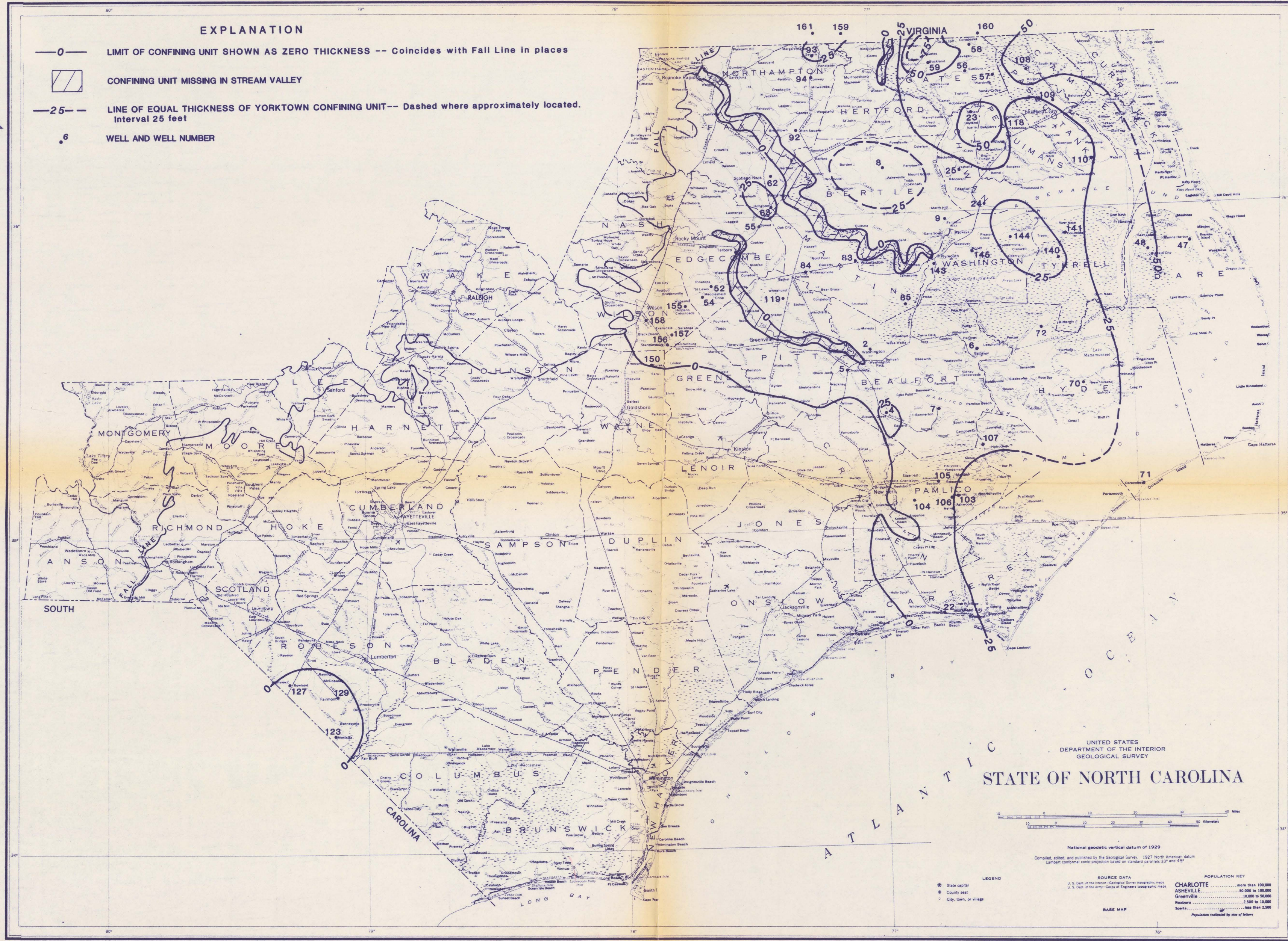
THICKNESS OF THE YORKTOWN CONFINING UNIT
