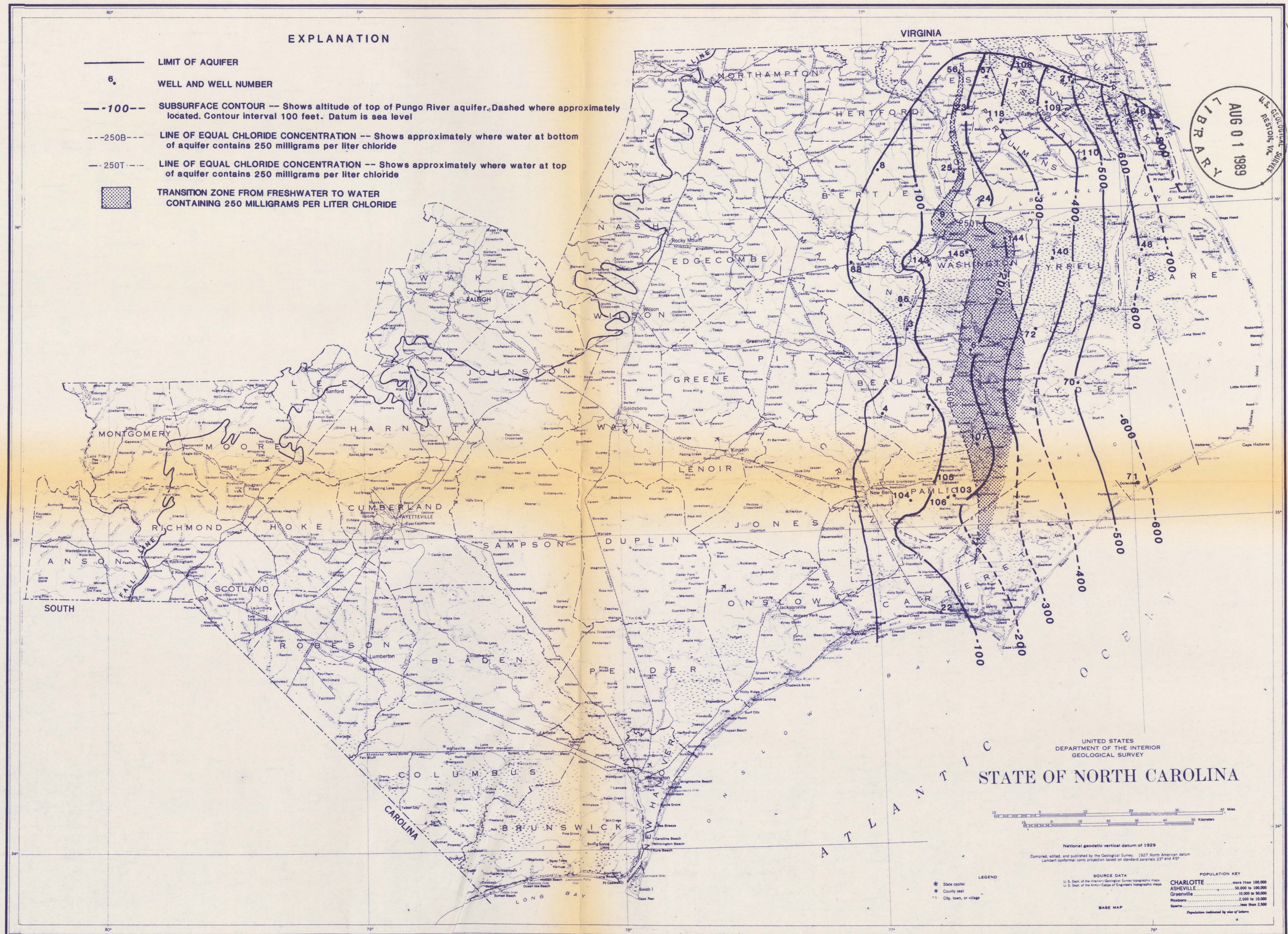
ALTITUDE OF THE TOP OF THE PUNGO RIVER AQUIFER
