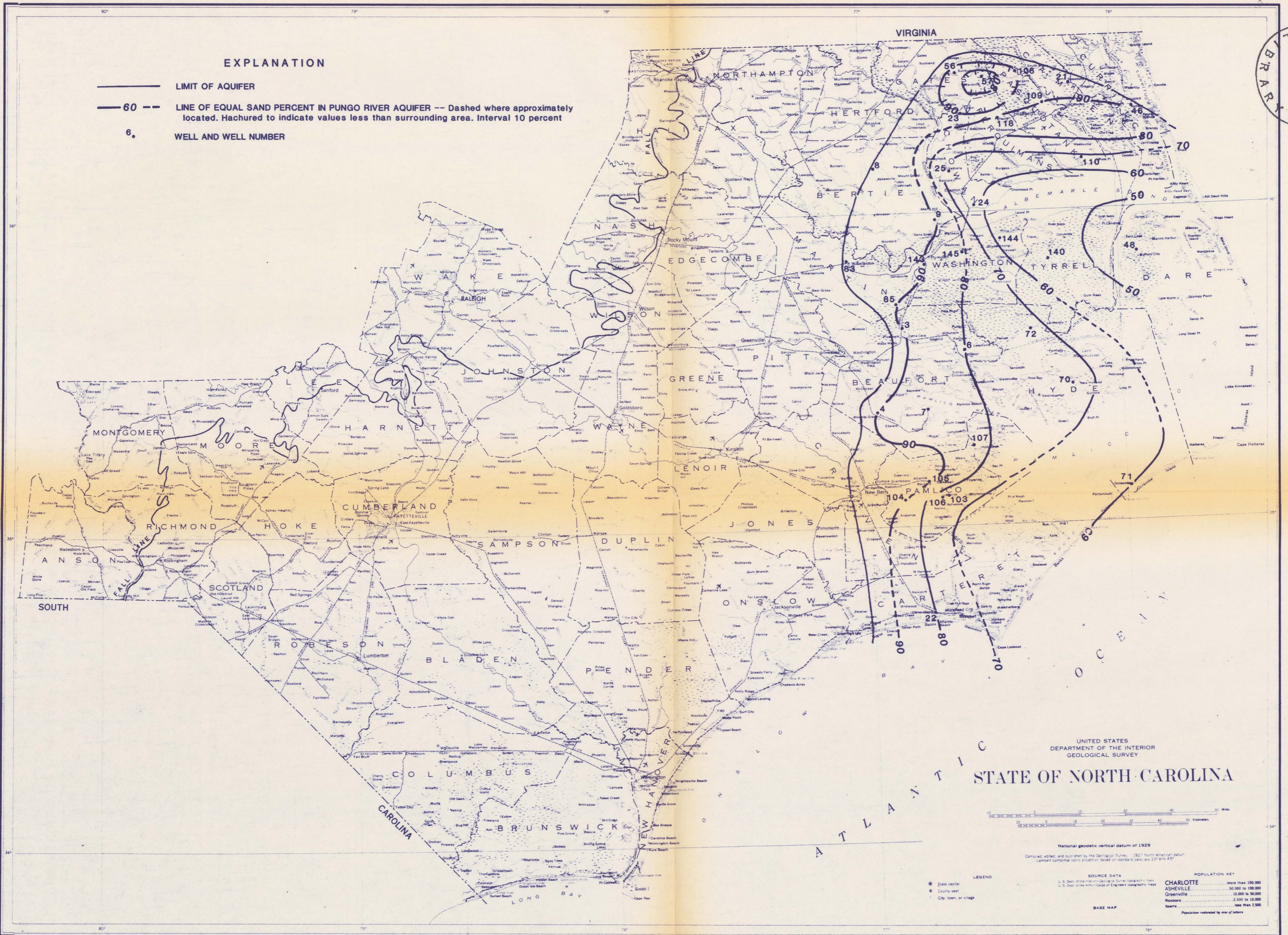
SAND PERCENTAGE IN THE PUNGO RIVER AQUIFER
