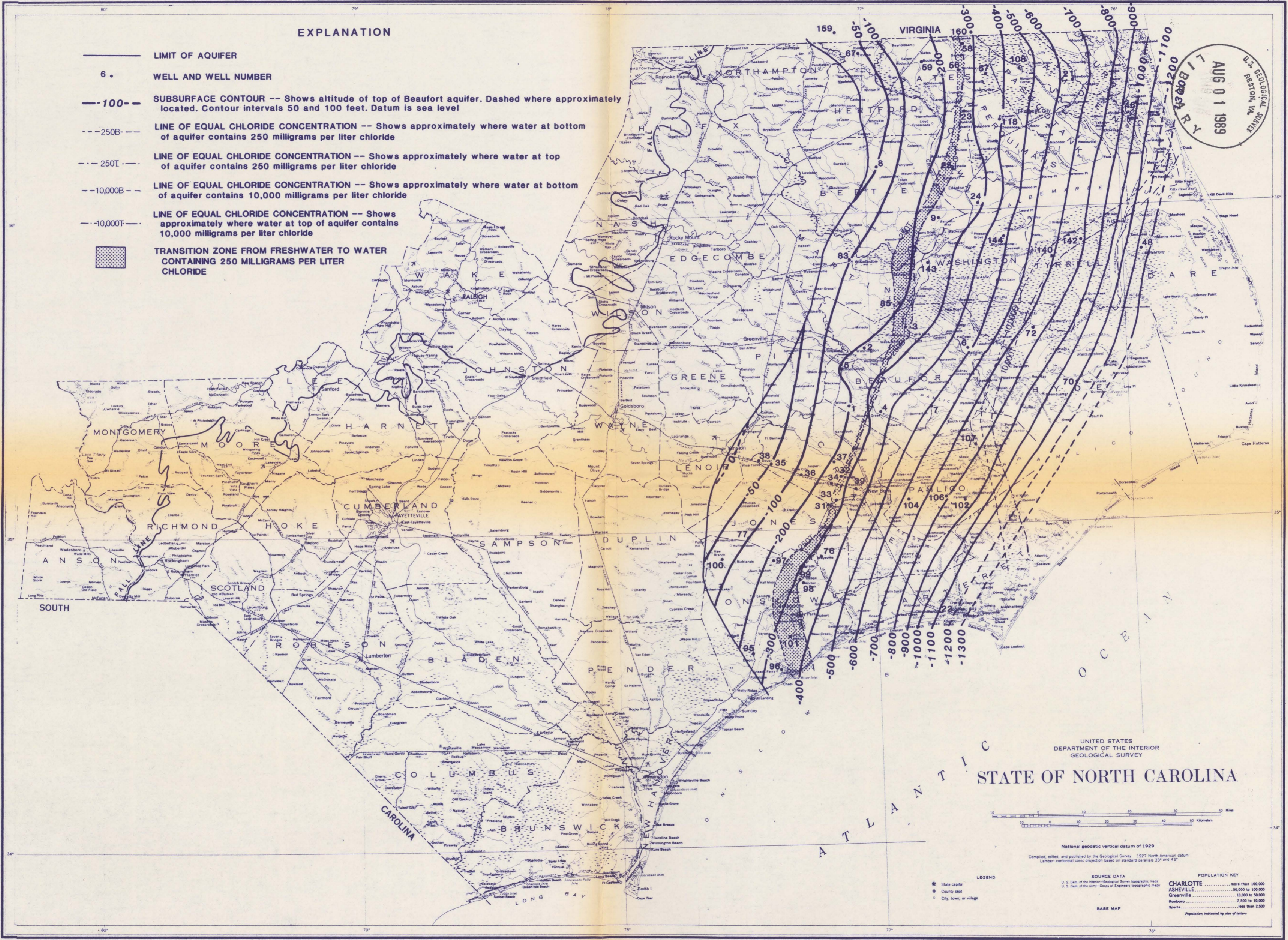
ALTITUDE OF THE TOP OF THE BEAUFORT AQUIFER
