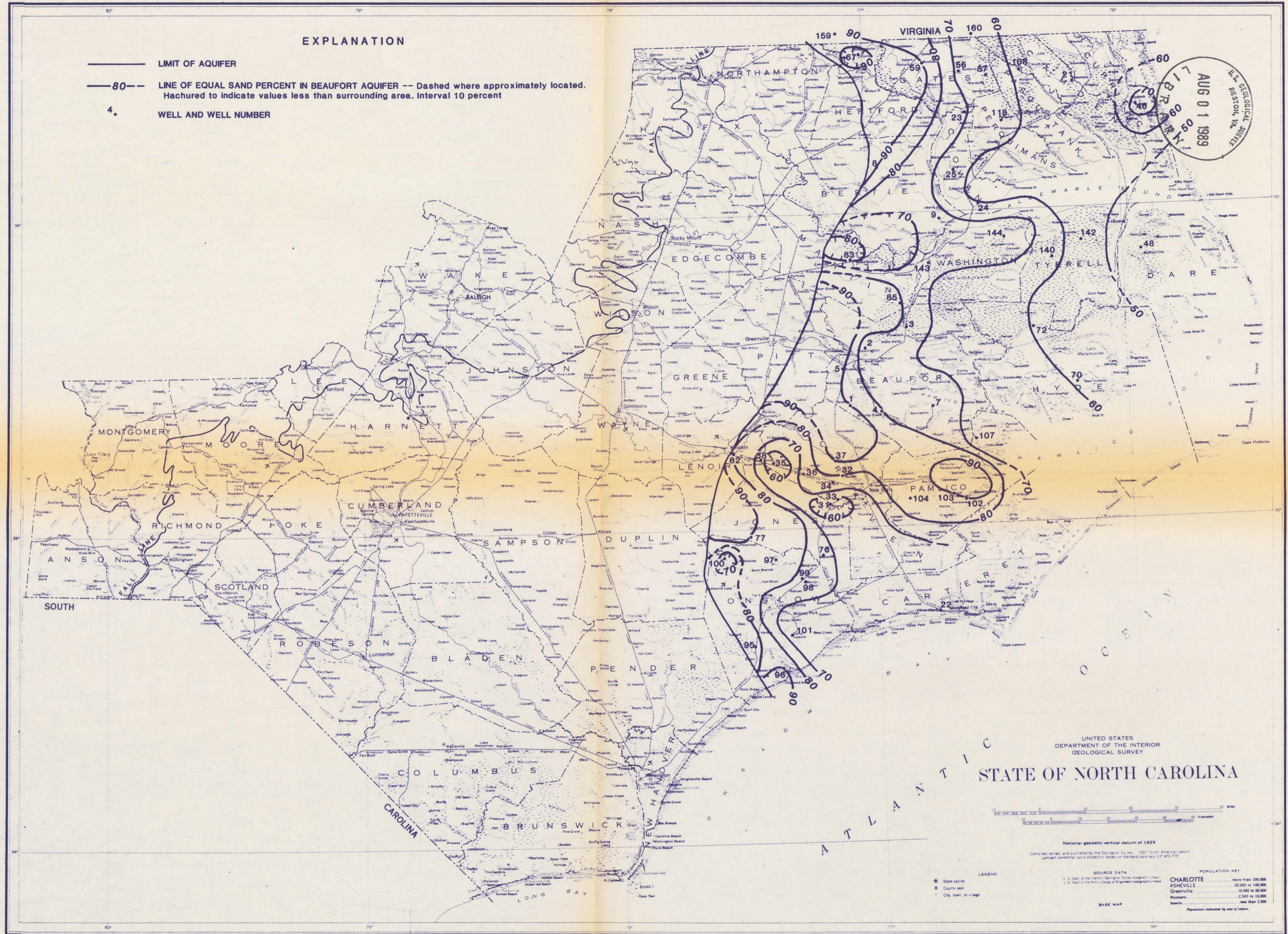
SAND PERCENTAGE IN THE BEAUFORT AQUIFER
