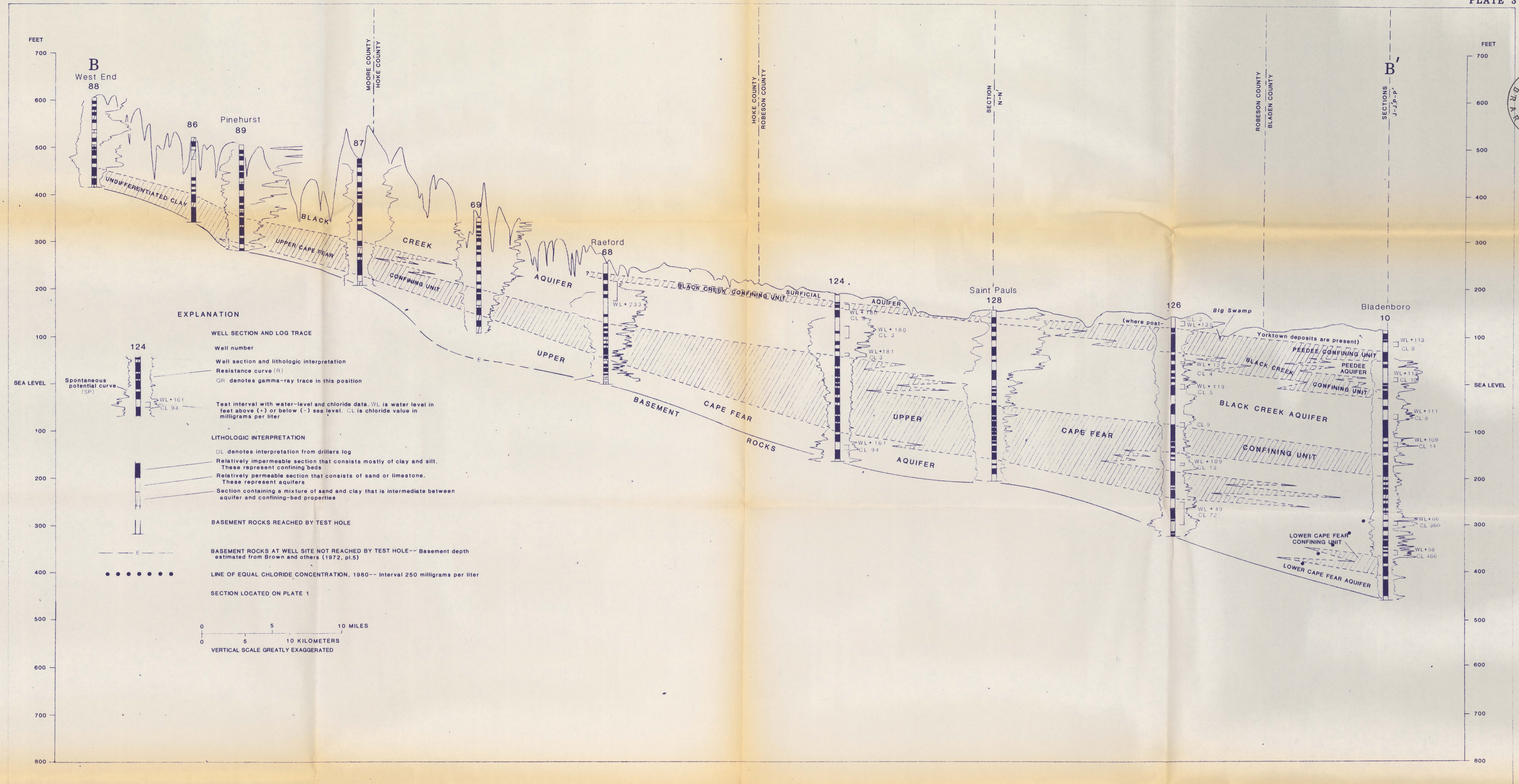
HYDROGEOLOGIC SECTION B-B' FROM WEST END, MOORE COUNTY TO BLADENBORO, BLADEN COUNTY
